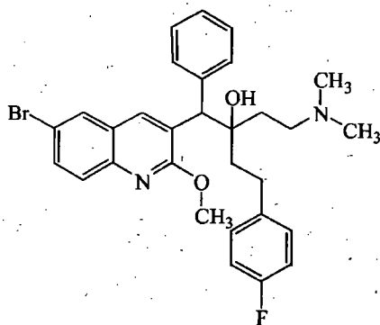
Compound 27 (B1)
