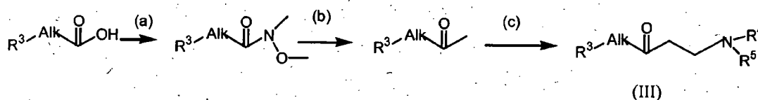
15 Scheme 4
