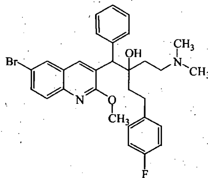
Compound 28 (B2)
