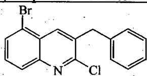
intermediate 6
