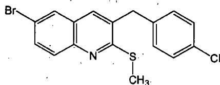
Intermediate 19
