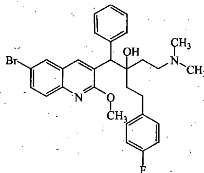
Compound 26 (A2)
