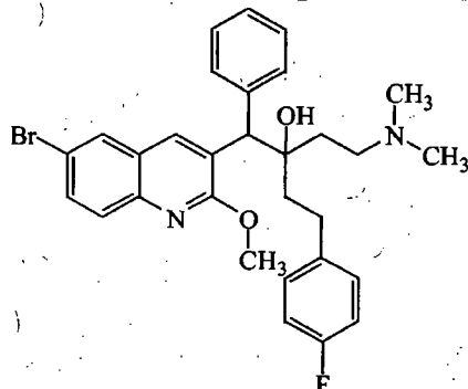
Compound 25 (A1)
