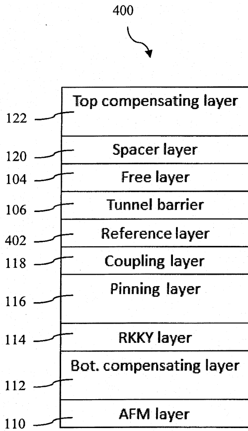
Bottom pinned MTJ
