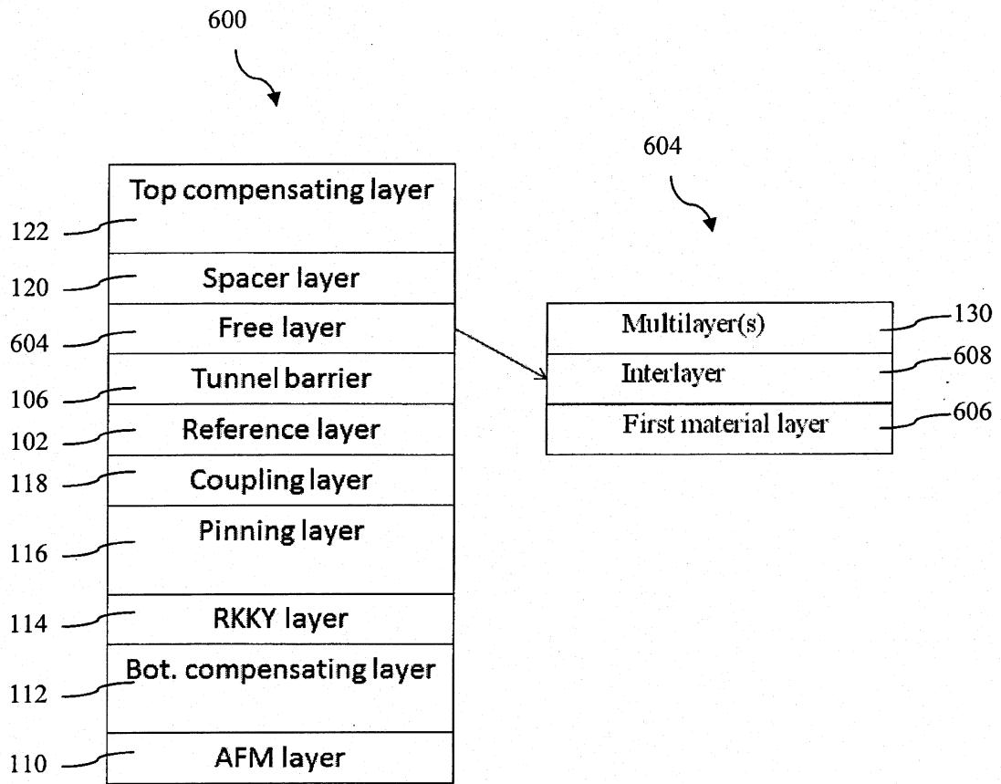
Bottom pinned MTJ
