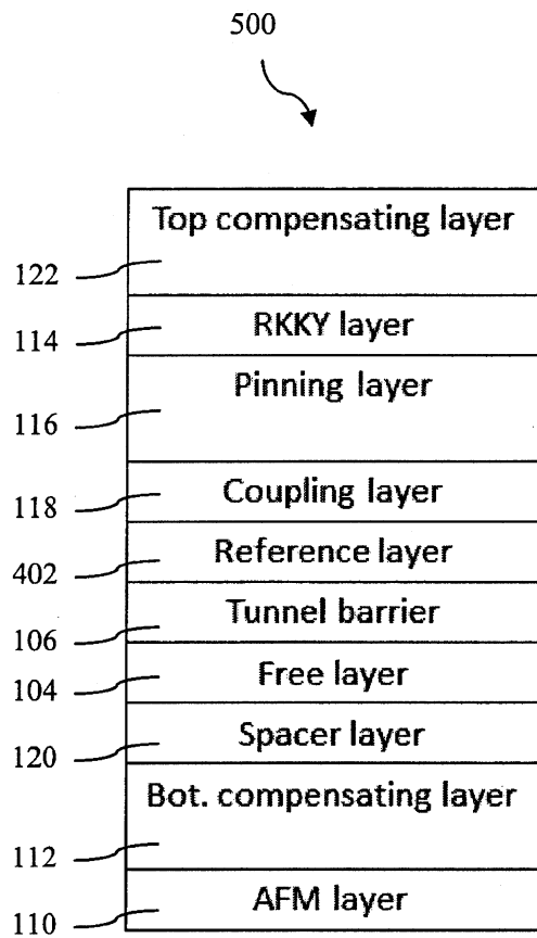
Top pinned MTJ
