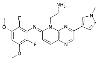
compound 68
