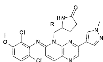
compound 92
