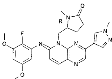
compound 160
