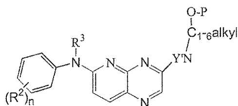
(XXVI)
