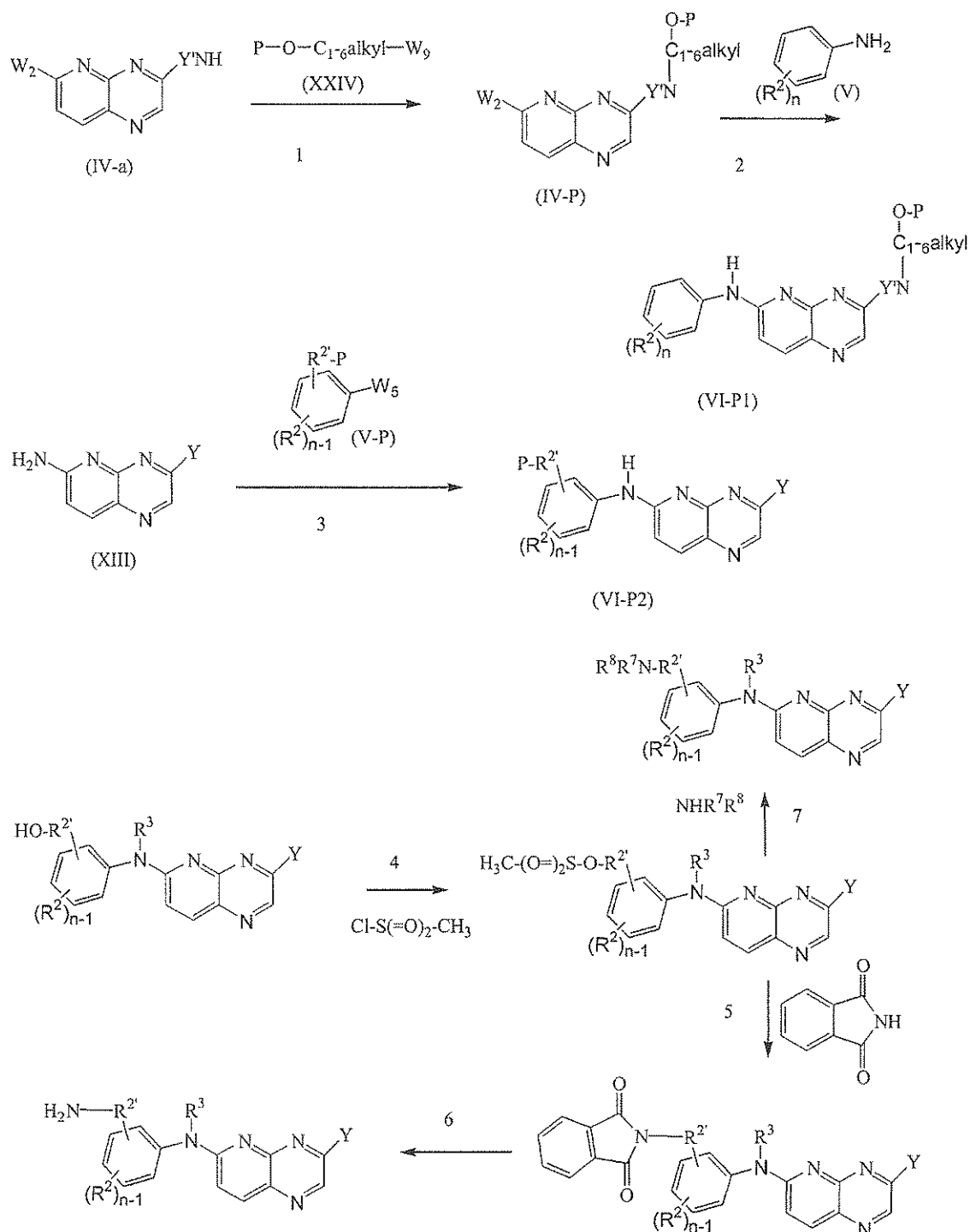
Scheme 9
