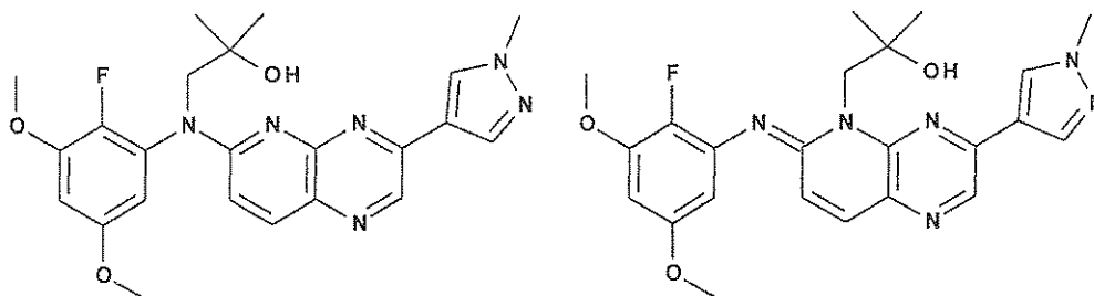
compound 245
