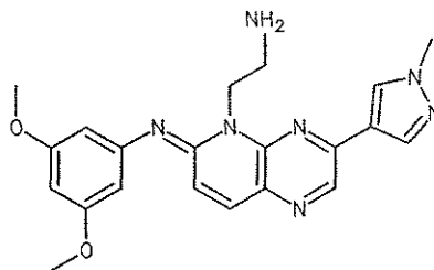
and compound 237
