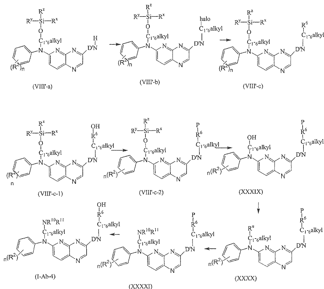
Scheme 4
