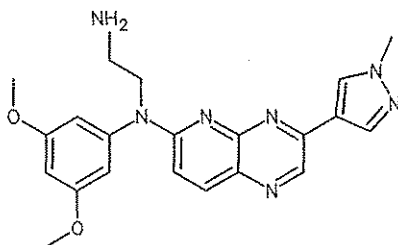
compound 236
