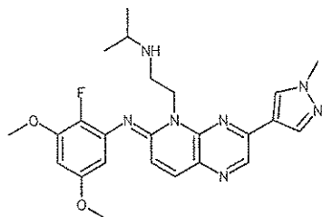
Compound 37
