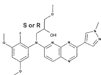
compound 59
