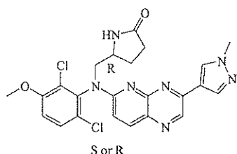
compound 94
