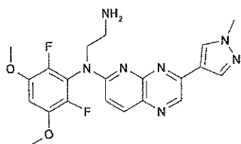
Compound 67
