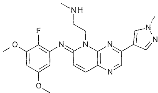
compound 38
