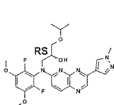
compound 61
