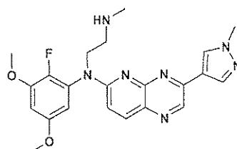
and compound 39
