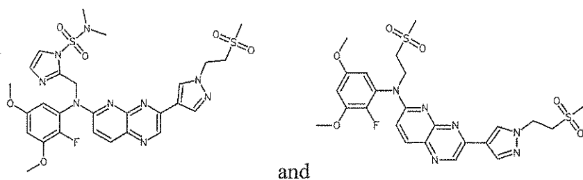
compound 265
