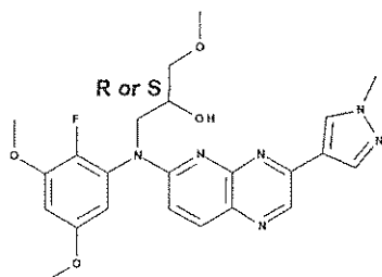
compound 58
