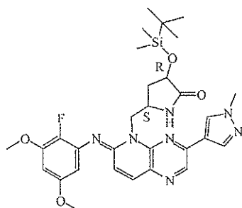
intermediate 125
