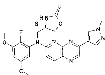
Compound 111
