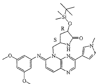
intermediate 128
