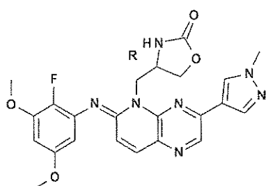
compound 123
