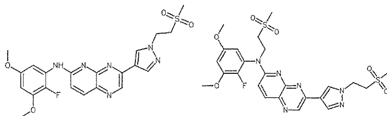
Intermediate 123
