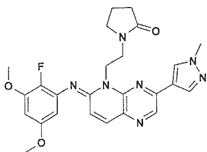
compound 156
