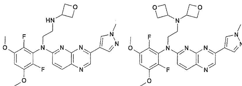
compound 162
