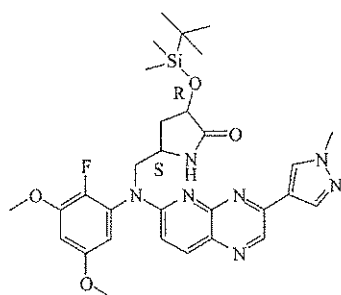
intermediate 126
