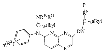
(XXXXI)
