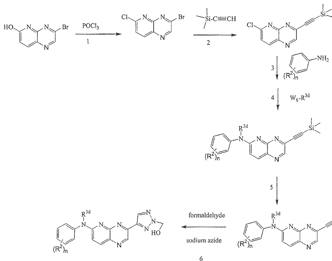
Scheme 11
