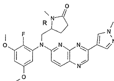
and compound 161
