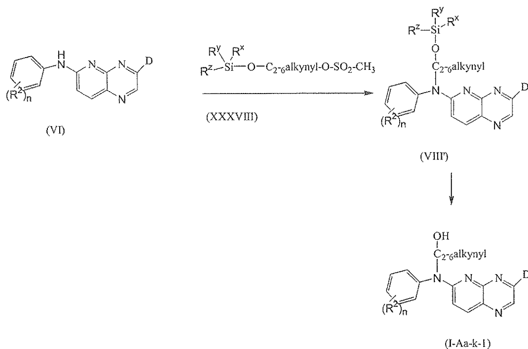
Scheme 1C
