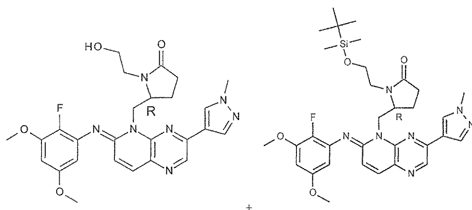
Intermediate 111
