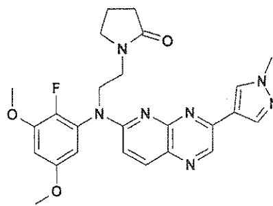
and compound 157
