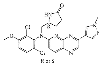
compound 93
