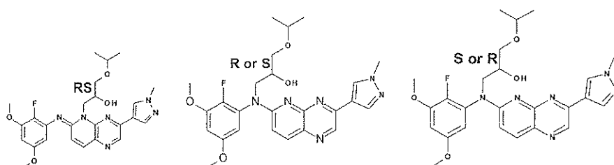
Compound 77
