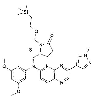
intermediate 58
