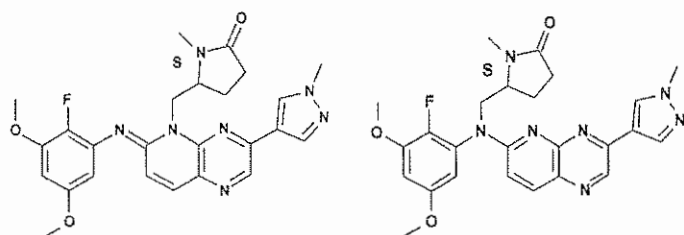
compound 158
