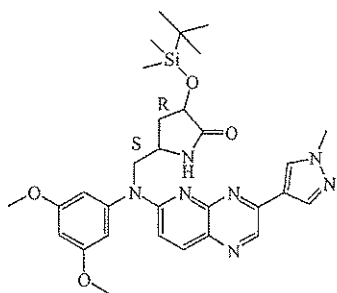
intermediate 127
