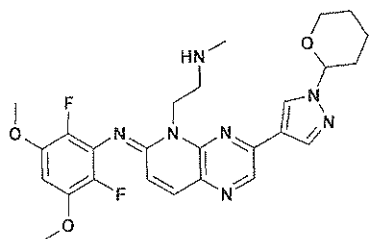
compound 107
