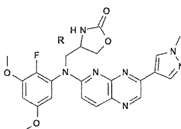
and compounds 124
