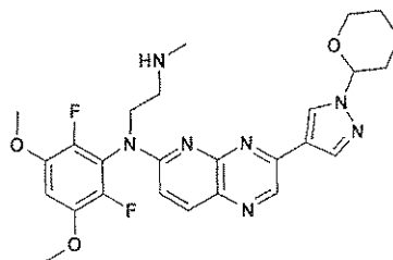
and compound 108
