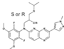
compound 62
