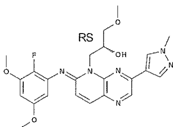
compound 60
