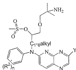
(XXXV)
