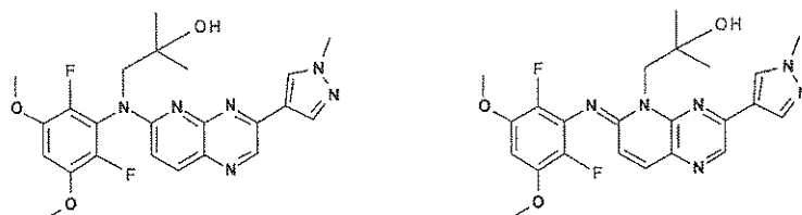
compound 278
