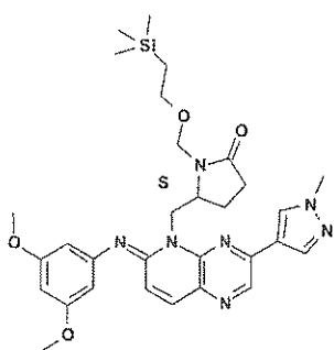
Intermediate 67
