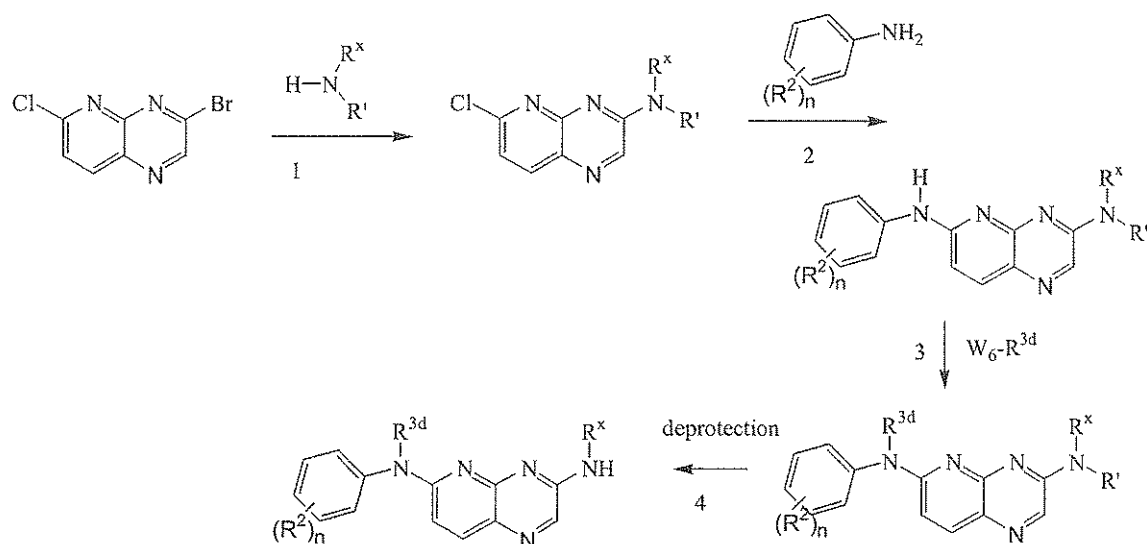
Scheme 12
