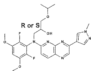
compound 63
