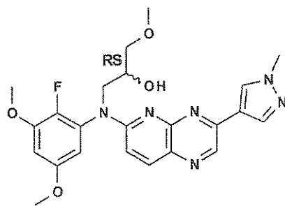
compound 57
