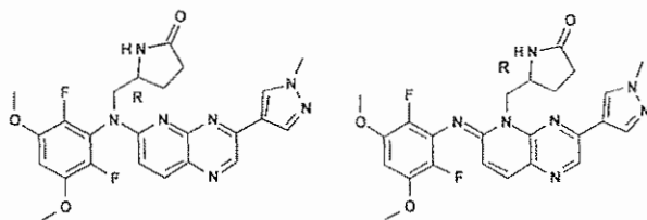
Compound 192
