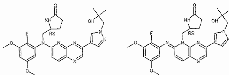
compound 285
