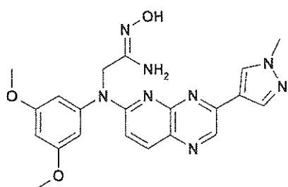
Intermediate 63
