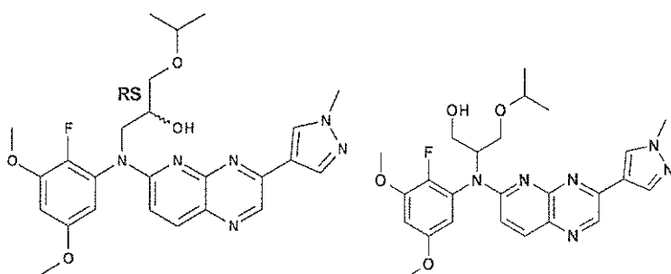
Compound 75
