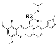
and compound 64
