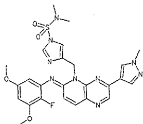
compound 35
