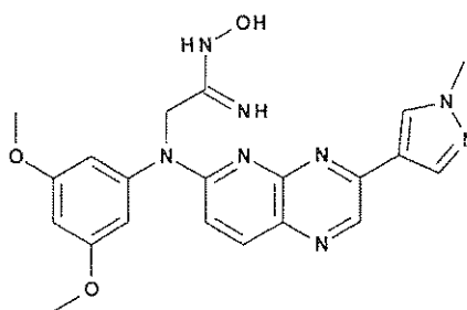
and Intermediate 64
