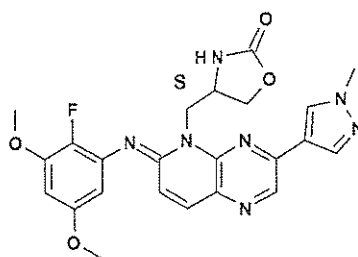
and compound 112
