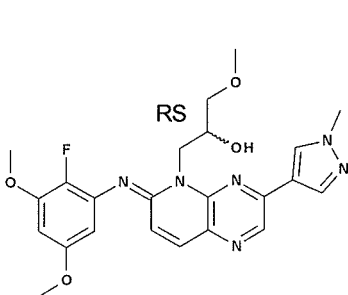
compound 60
