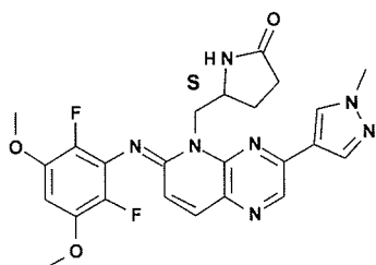
compound 47
