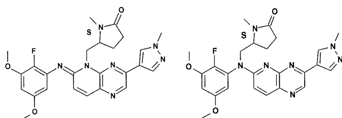
compound 159
