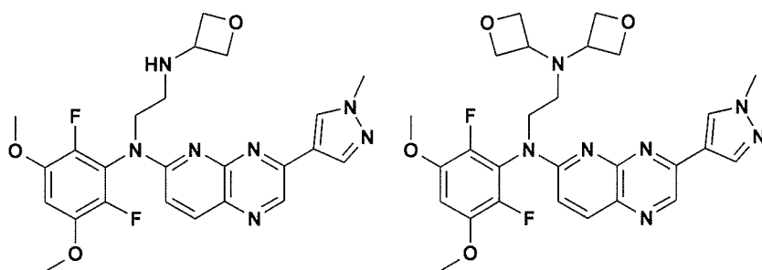
compound 162
