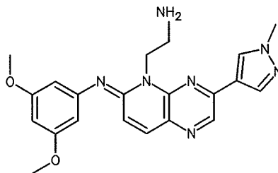
compound 237
