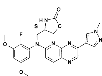
Compound 111
