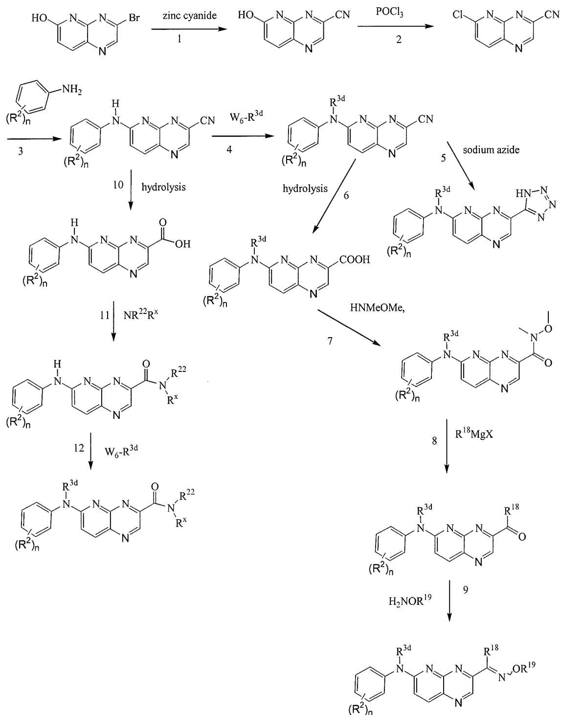
Scheme 10
