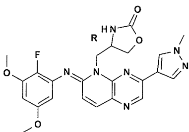
compound 123
