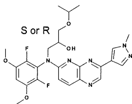
compound 62
