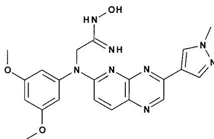
and Intermediate 64
