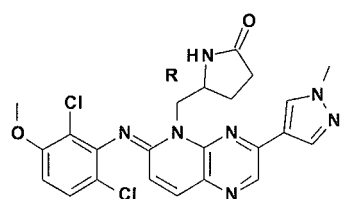
compound 92
