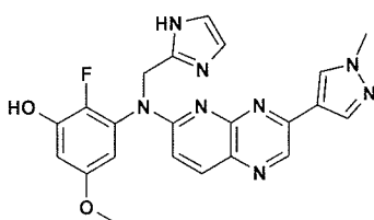
Preparation of compound 95
