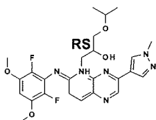
and compound 64
