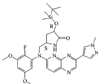
intermediate 126
