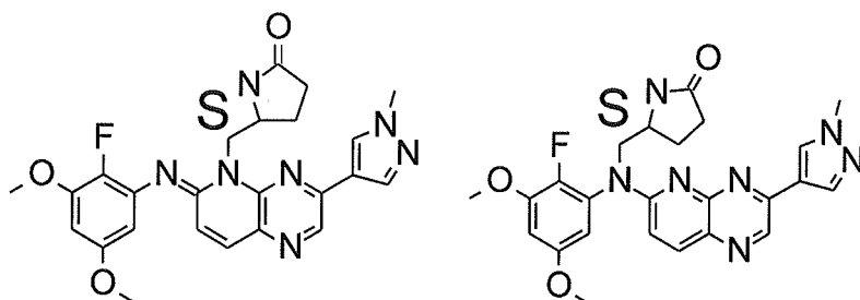
compound 45 and compound 46
