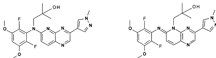
compound 278
