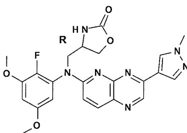
and compounds 124
