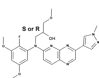
compound 59
