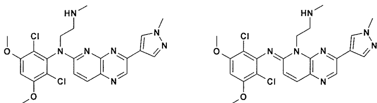
Compound 81 and compound 82
