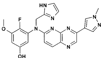
Preparation of compound 95
