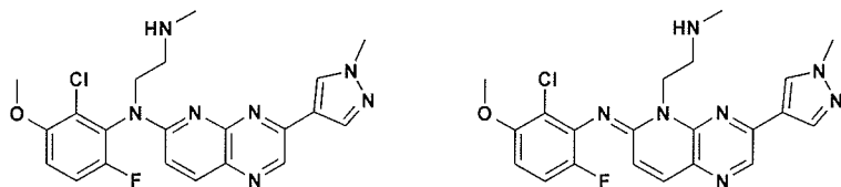
Compound 69 and compound 70
