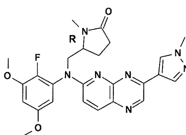
and compound 161
