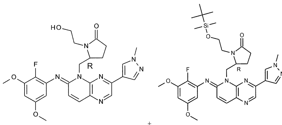
Intermediate 111
