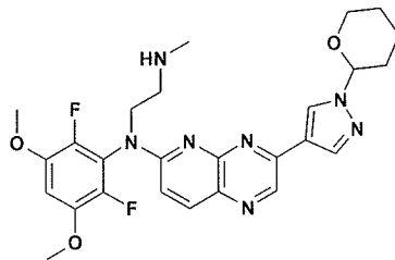
compound 108
