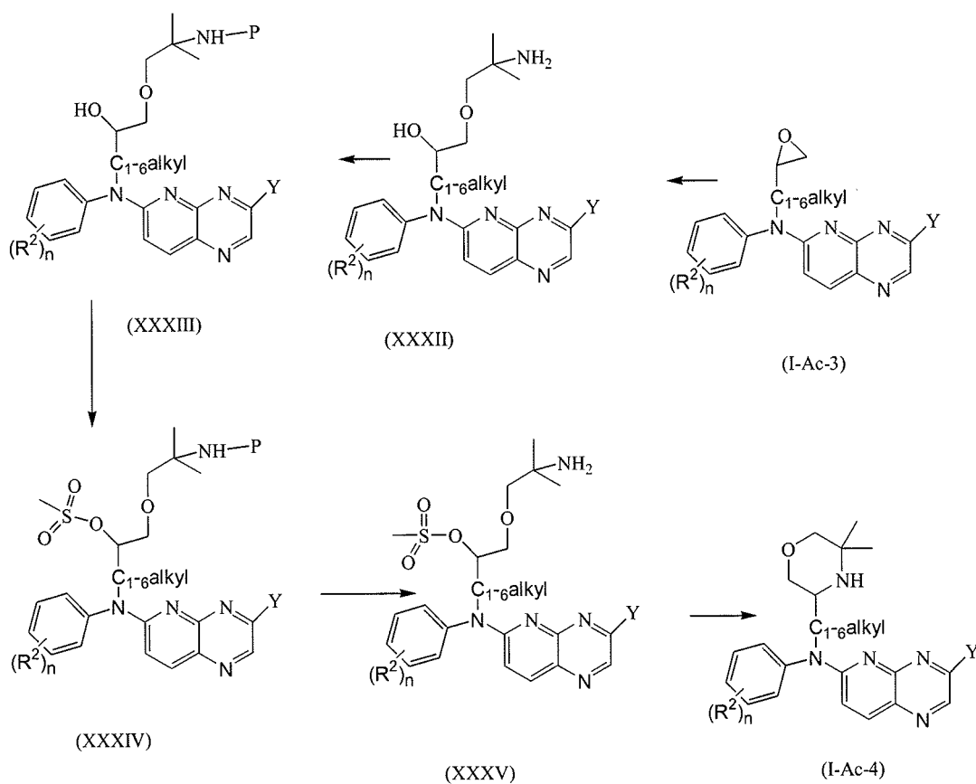
Scheme 7
