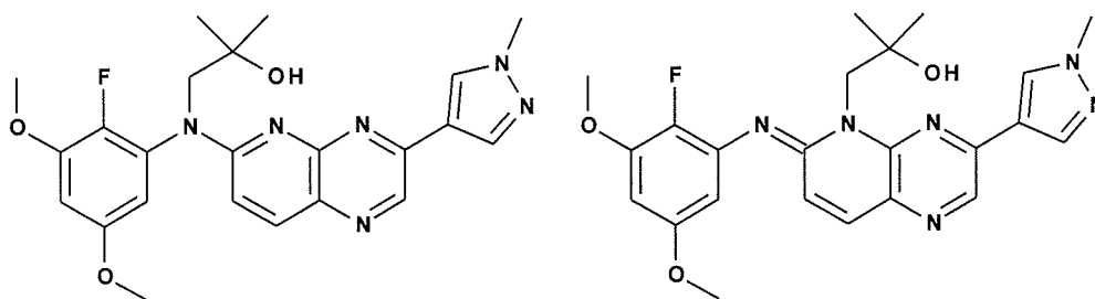
compound 245
