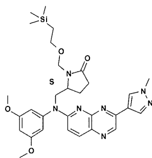
intermediate 58
