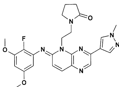
compound 156
