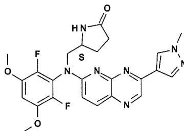
compound 48
