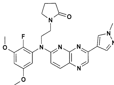
compound 157
