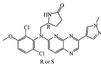
and compound 93
