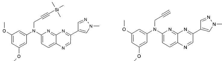
intermediate 13 and compound 22
