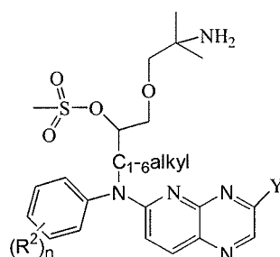
(XXXV)
