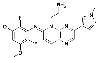
compound 68
