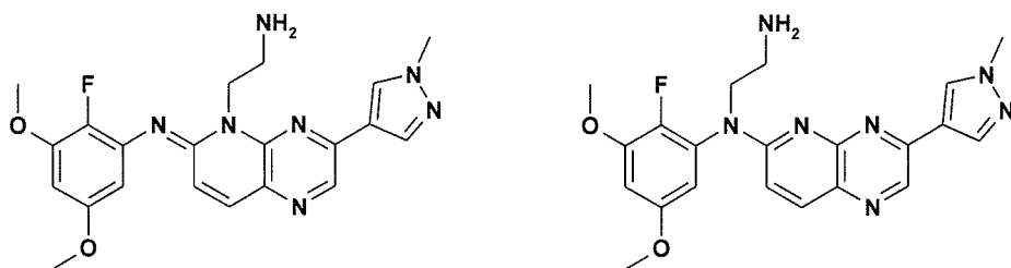
compound 167 and compound 168
