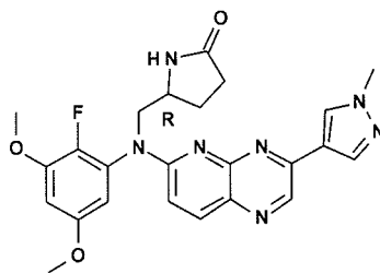
compound 53
