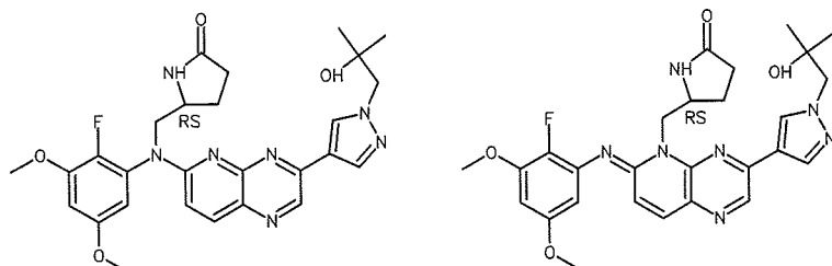
compound 286
