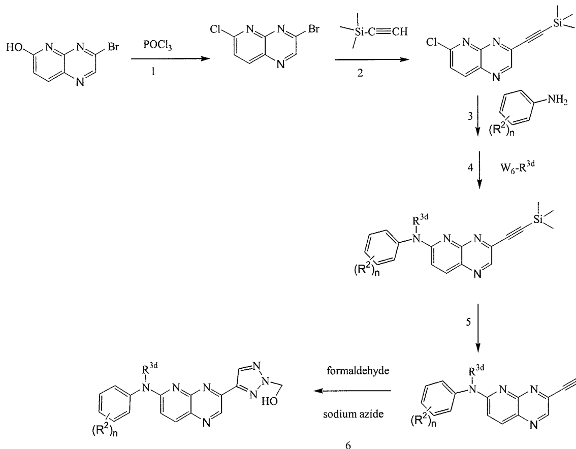
Scheme 11
