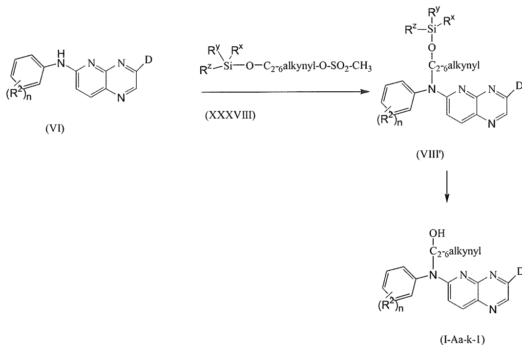
Scheme 1C
