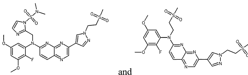
compound 265
