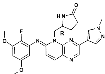
compound 52
