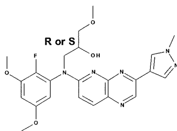
compound 58
