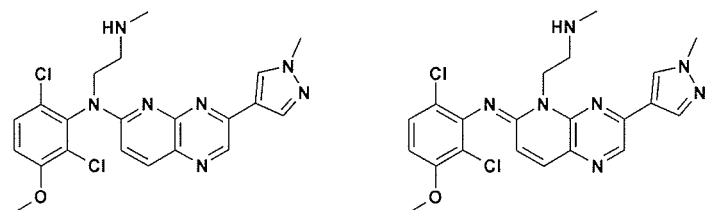
Compound 83 and compound 84
