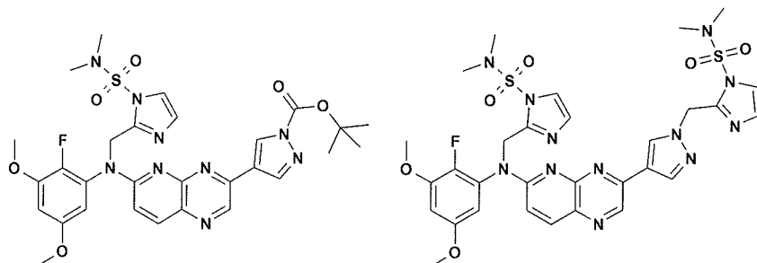
Compound 102
