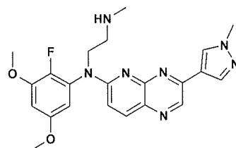
and compound 39
