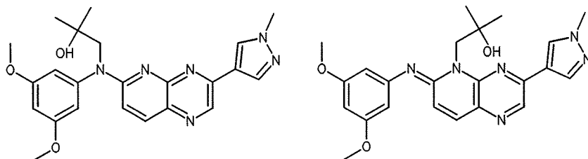
compound 276
