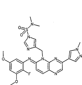
compound 35
