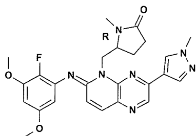
compound 160
