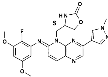
compound 112
