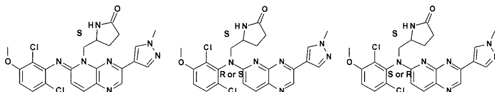
compound 89 and compound 90 and compound 91
