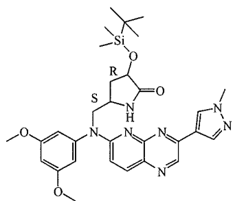
intermediate 127
