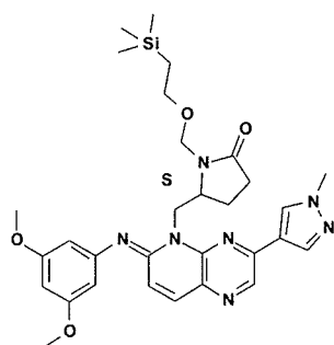
Intermediate 67
