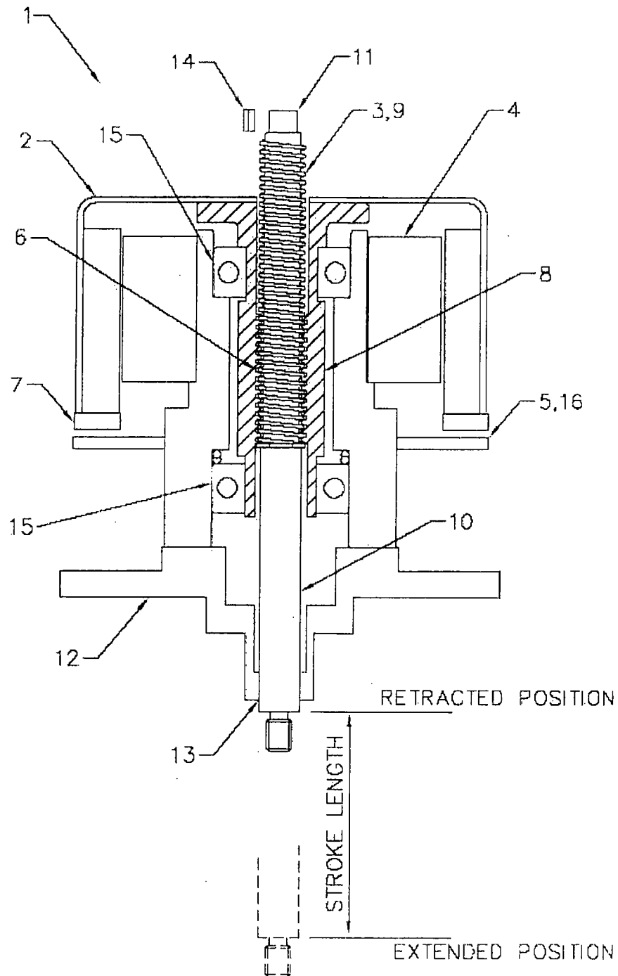
Drawing 1. Cross-sectional view of the linear actuator
