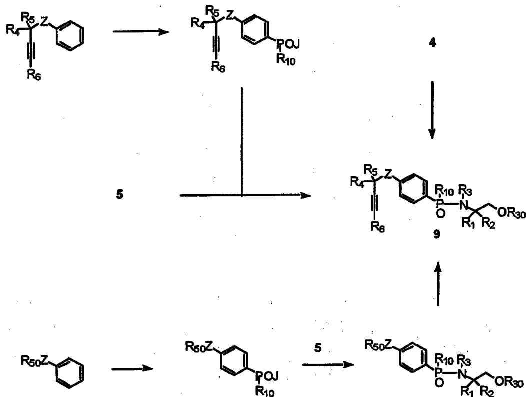
Scheme 5:
