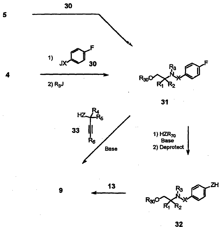
Scheme 8:
