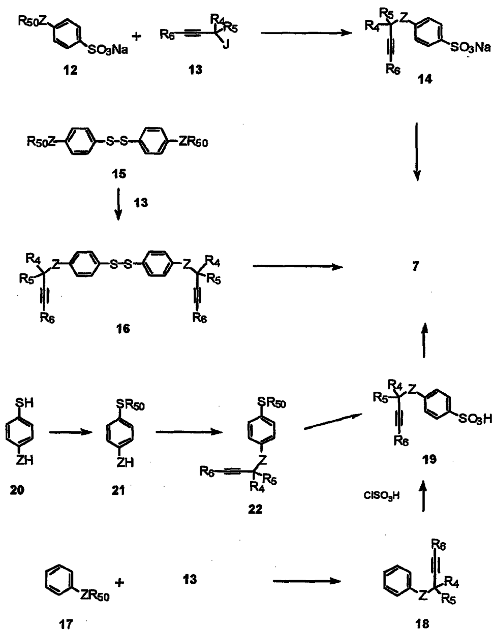
Scheme 4:
