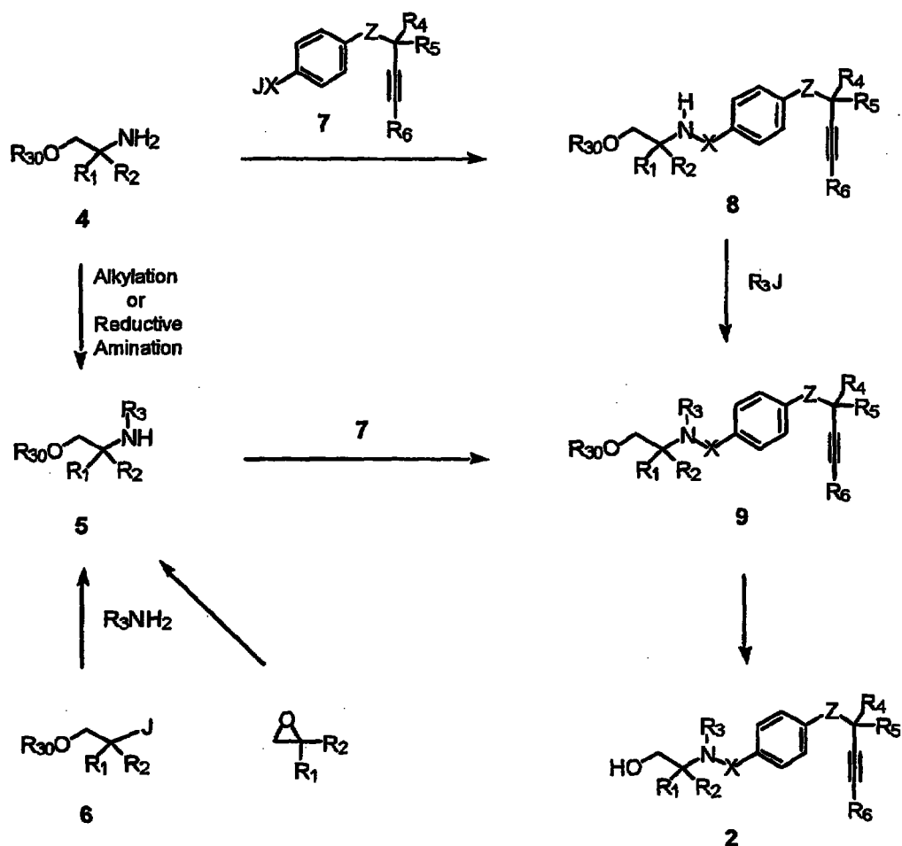
Scheme 2:
