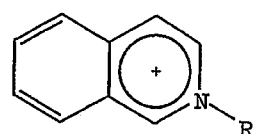
ISOQUINOLINIUM
