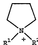
PYRROLIDINIUM
