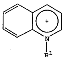
QUINOLINIUM
