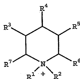
PIPERIDINIUM
