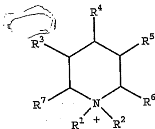
PIPERIDINIUM
