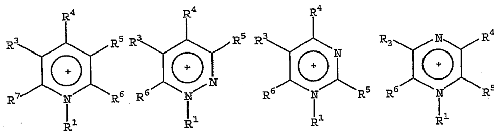
PYRAZINIUM
