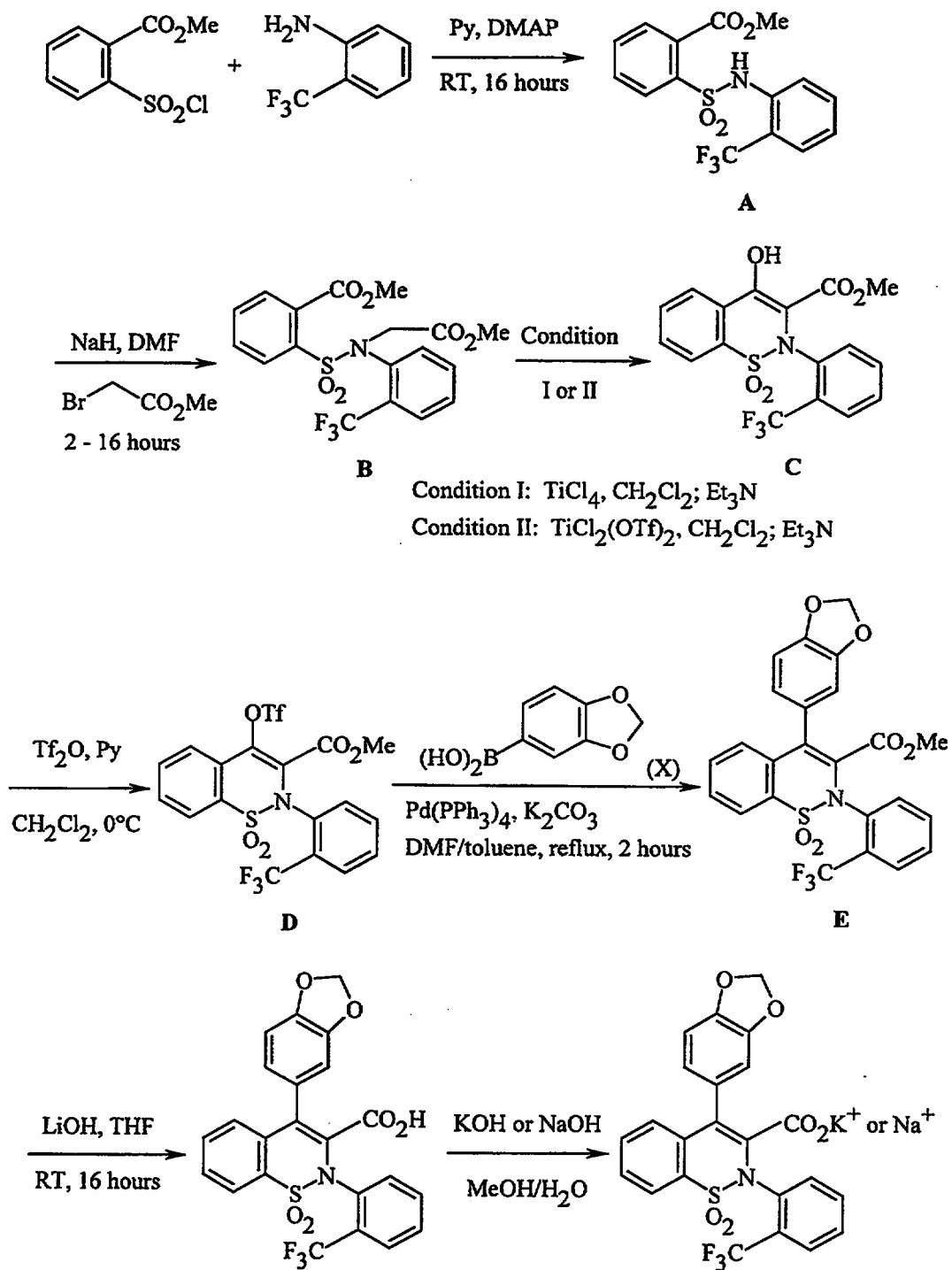
Scheme 1
