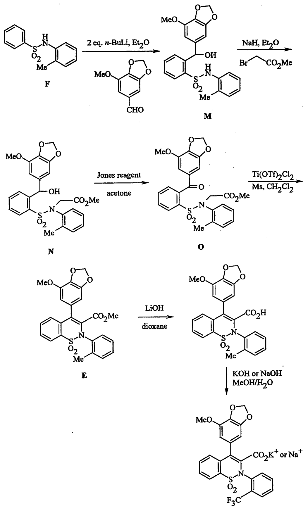
Scheme 3
