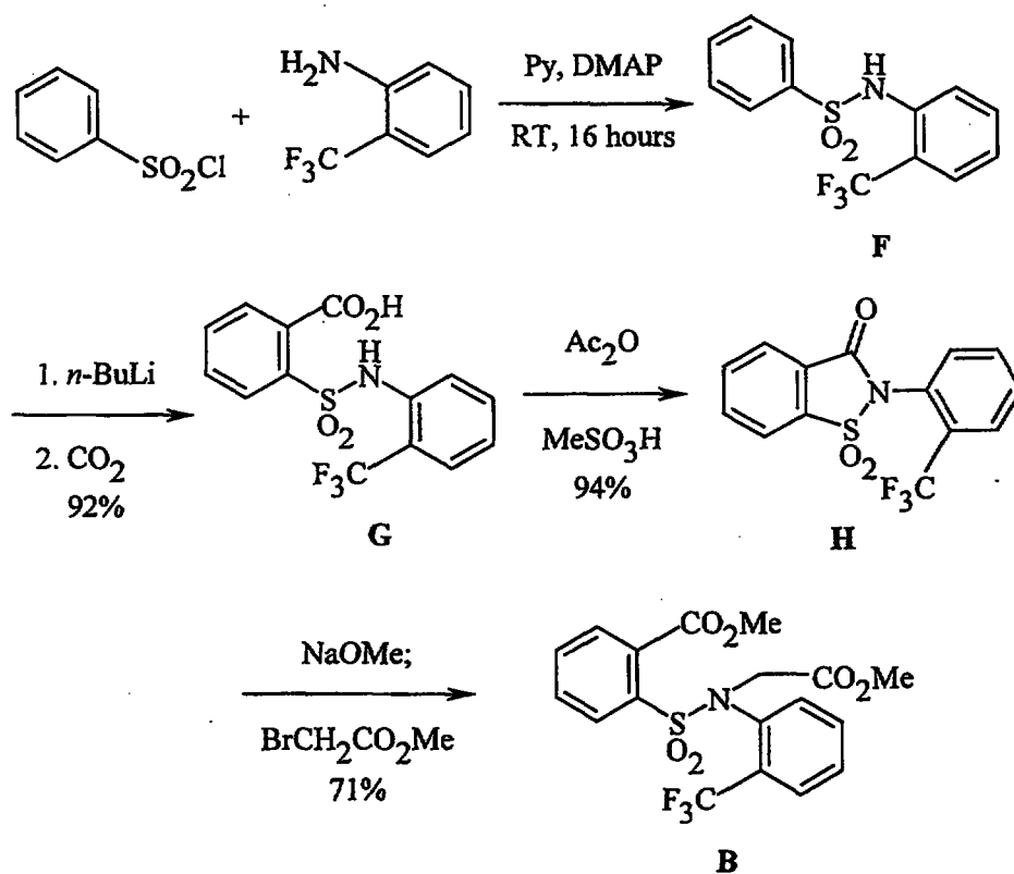
Scheme 1b
