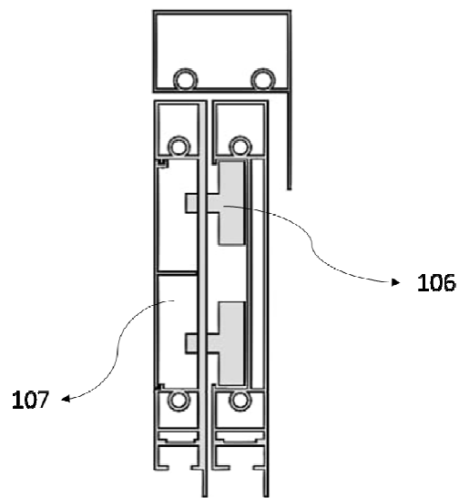
VIEW AA
