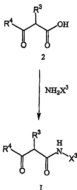
Reaction Scheme 2
