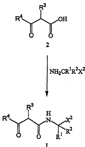
Reaction Scheme 1
