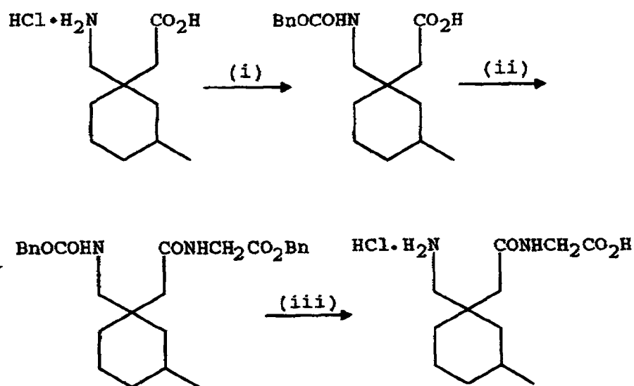
Scheme 8
