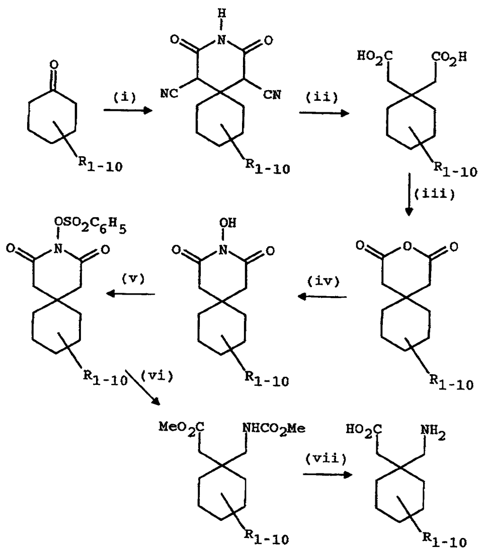
Scheme 4
