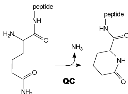
Scheme 2: Cyclization of L-homoglutamine by QC
