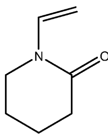
Formula V
