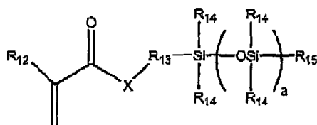
Formula VII
