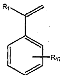
FORMULA X
