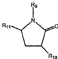
Formula IV
