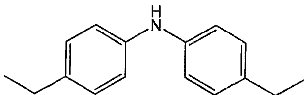
bis(4-ethylphenyl)amine
