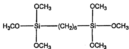
3,3,10,10-tetramethoxy-2,11-dioxa-3,10-disiladodecane
