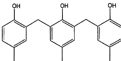
2,2'-((2-hydroxy-5-methyl-1,3-phenylene)bis(methylene))bis(4-methylphenol)
