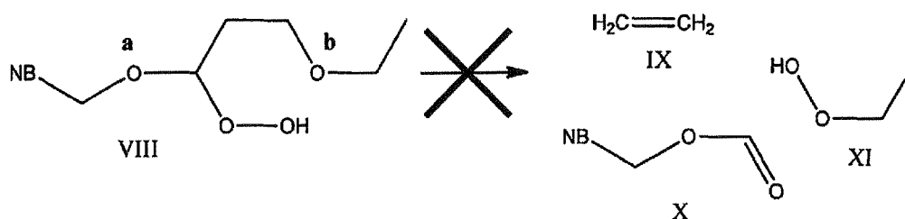
Scheme C
