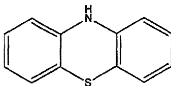
10H-Phenothiazine
