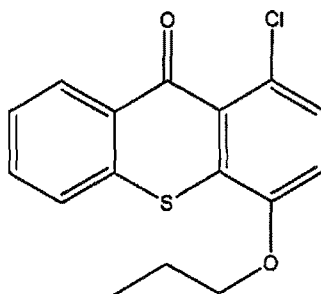
1-chloro-4-propoxy-9H-Thioxanthen-9-one
