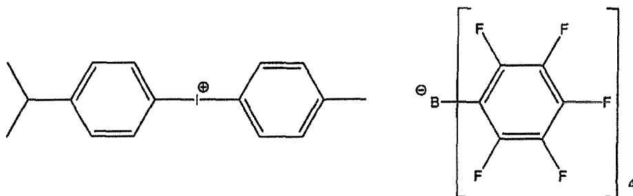
tetrakis(2,3,4,5,6-pentafluorophenyl)borate(1-)[4-(1-methylethyl)phenyl] (4-methylphenyl)-Iodonium
