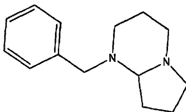
1-benzyl-octahydropyrrolo[1,2-a]pyrimidine
