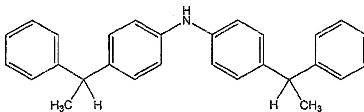
bis(4-(1-phenylethyl)phenyl)amine
