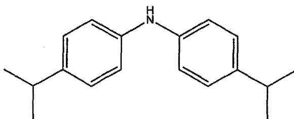
bis(4-isopropylphenyl)amine
