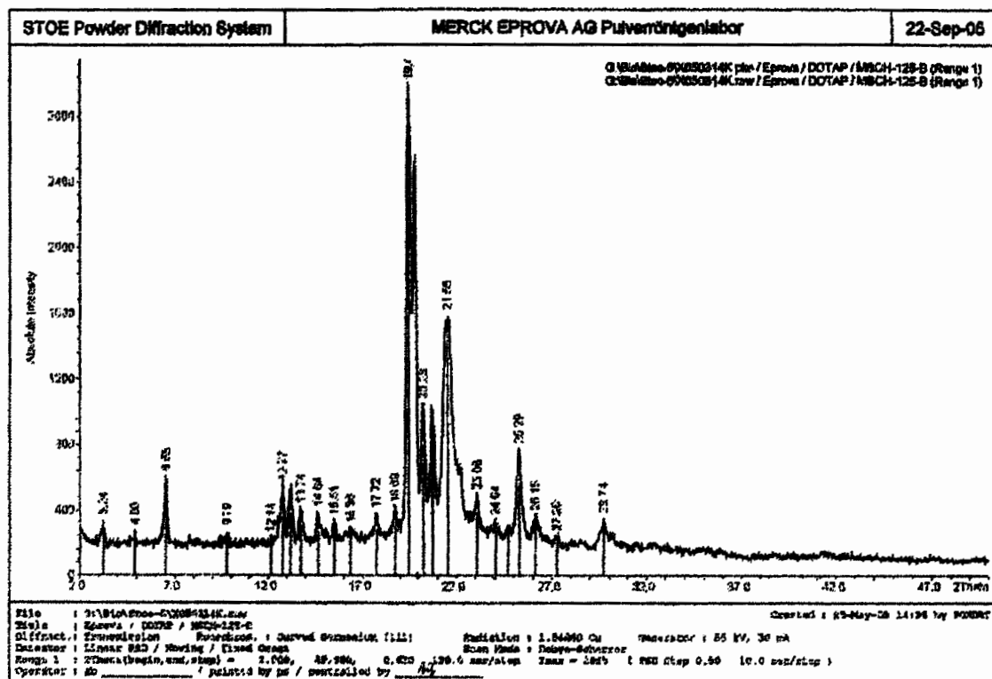
Figure 4: (type IV)
