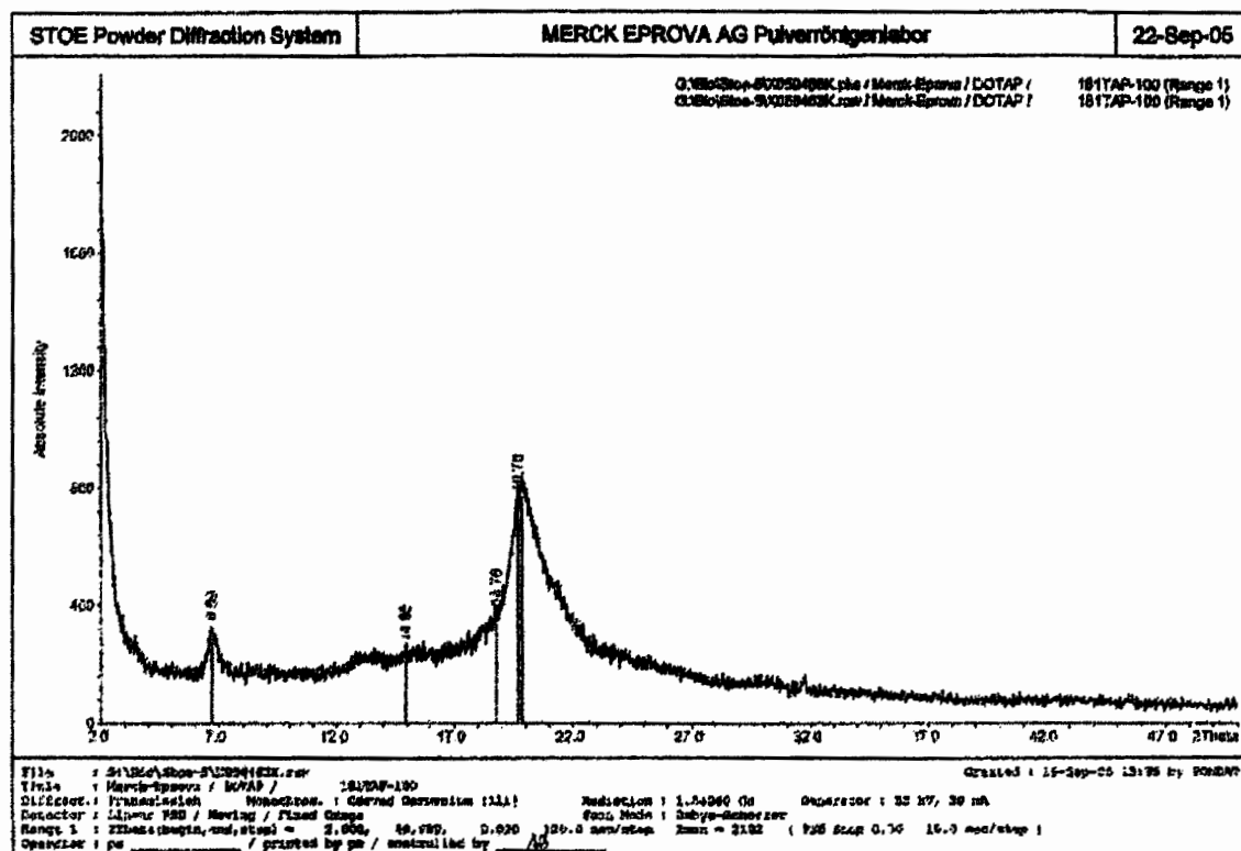
Figure 5: (amorphous)
