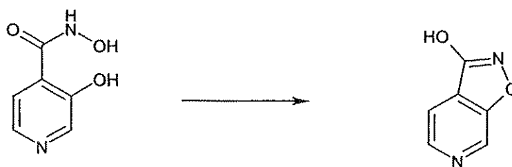
Isoxazolo[5,4-c]pyridin-3-ol (HIP)
