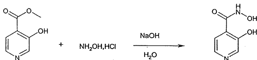
3,N-Dihydroxy-isonicotinamide
