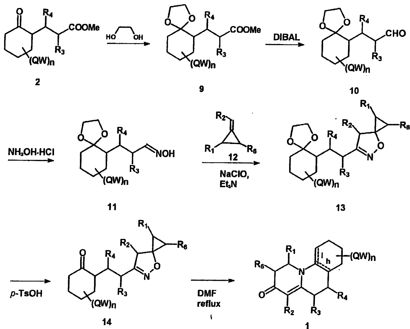
Scheme 2
