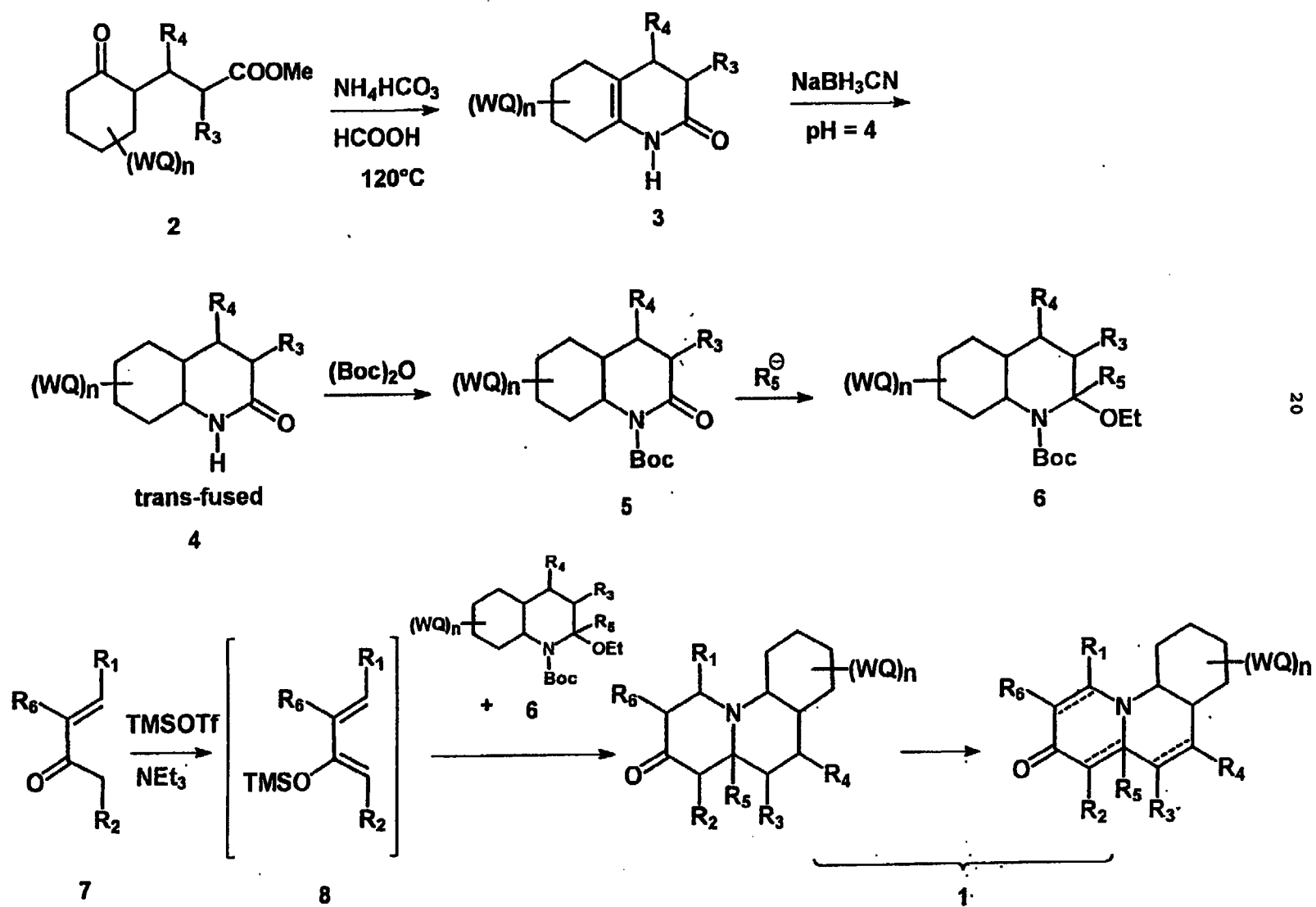
Scheme 1
