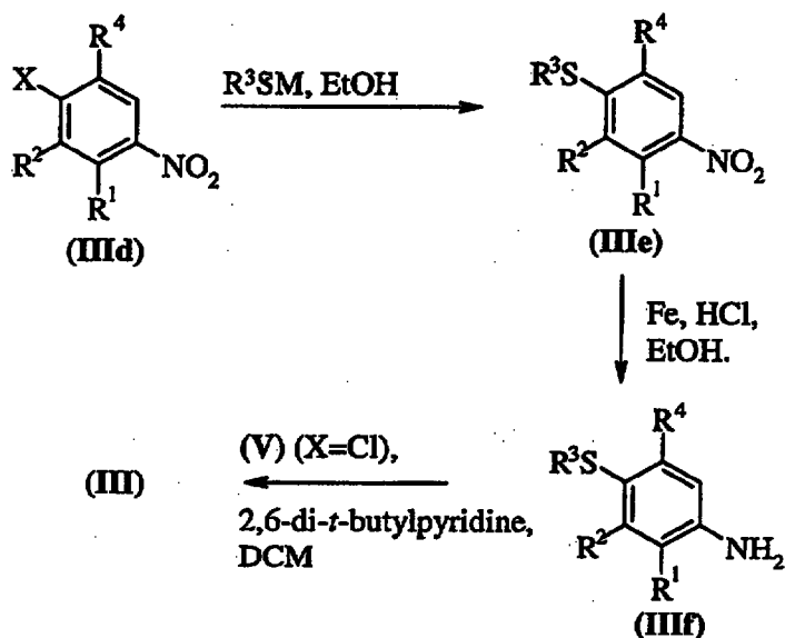
Scheme 3
