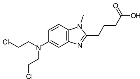
Bendamustine
