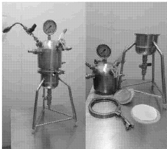
Figure 2: Representative image of lab scale pressure filter
