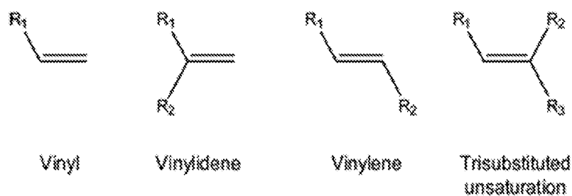
Scheme 1. General structures and nomenclature of unsaturations in polyolefins
