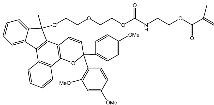
5 Photochromic compound III
