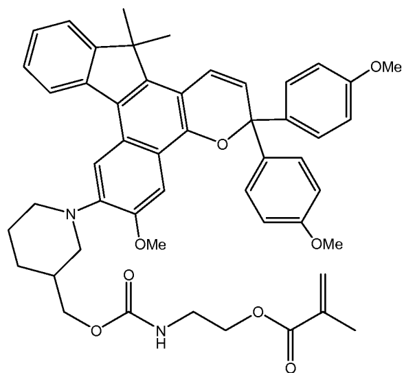
5 Photochromic compound III
