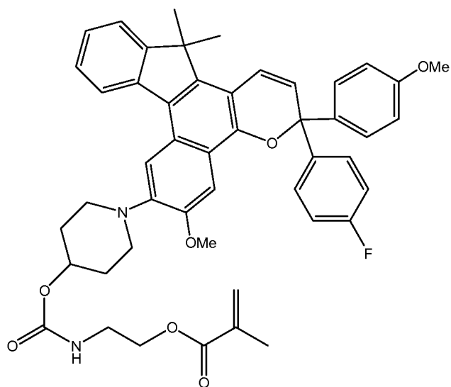
Photochromic compound VII
