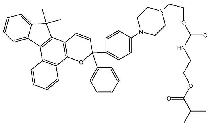
Photochromic compound VII
