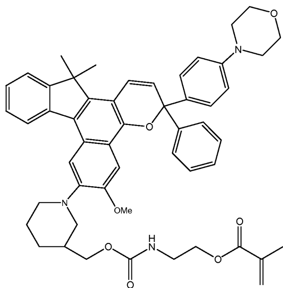
5 Photochromic compound V
