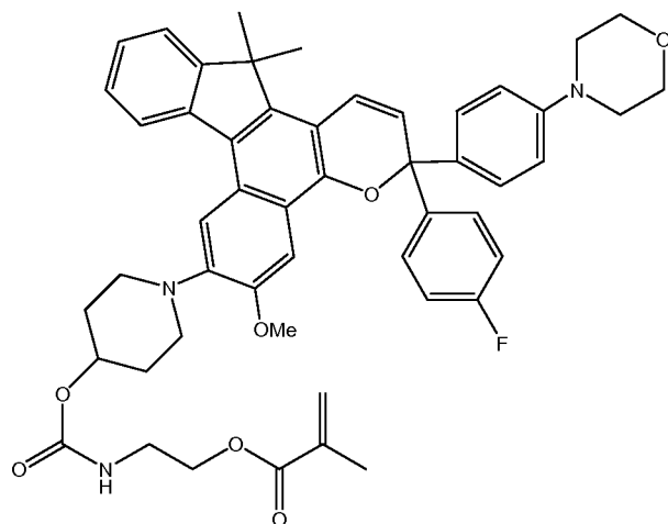
5 Photochromic compound IX
