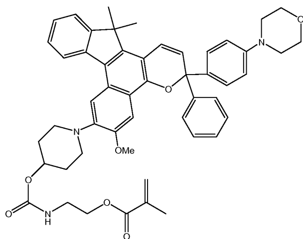
Photochromic compound XI
