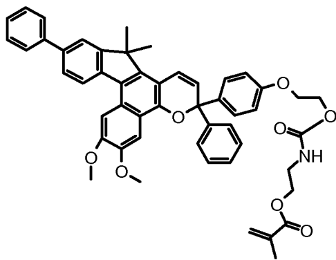
Photochromic compound XII
