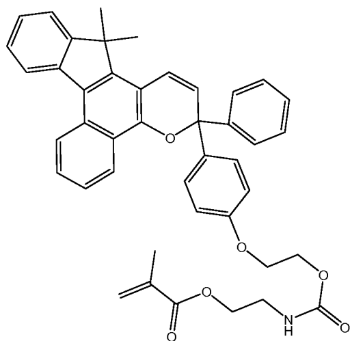
Photochromic compound X
