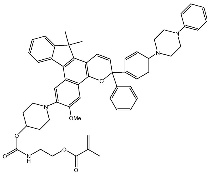
5 Photochromic compound V
