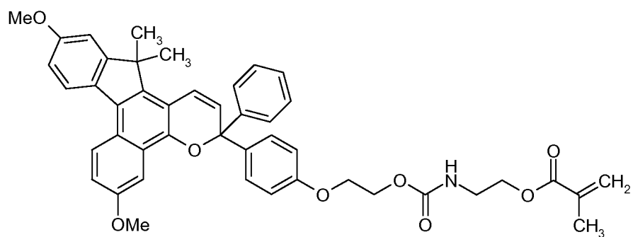
Photochromic compound II
