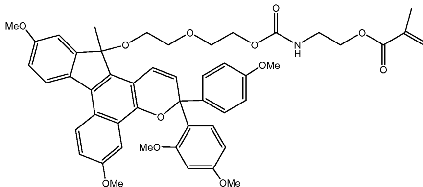
Photochromic compound I
