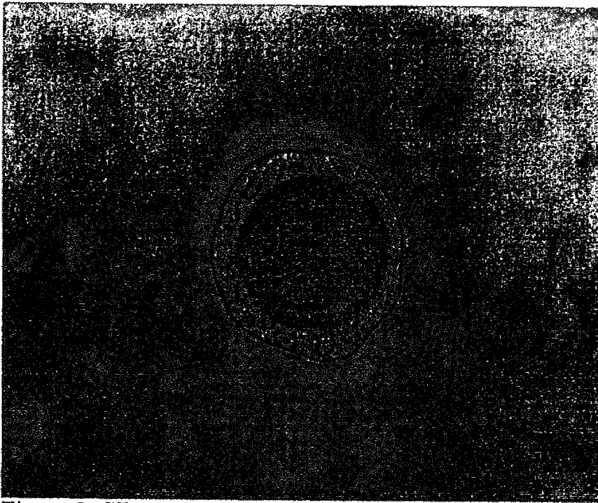
Figure 3: Silver plated copper 1xreflow pull test - breaks at first ball bond.
