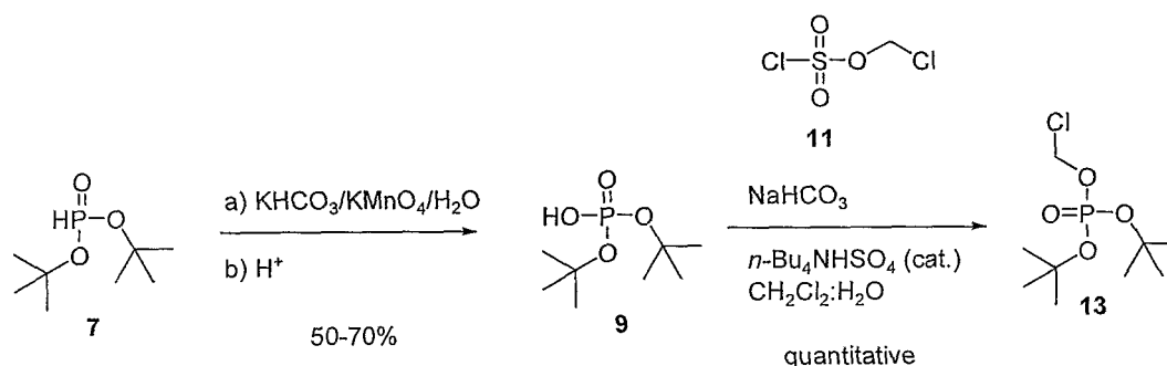
Scheme (III)
