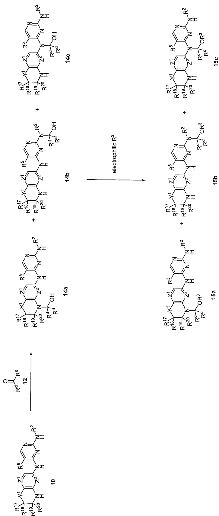
Scheme (I)
