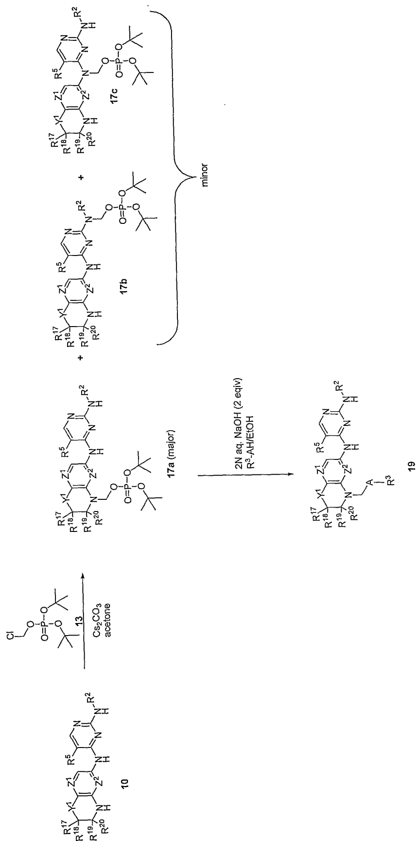
Scheme II
