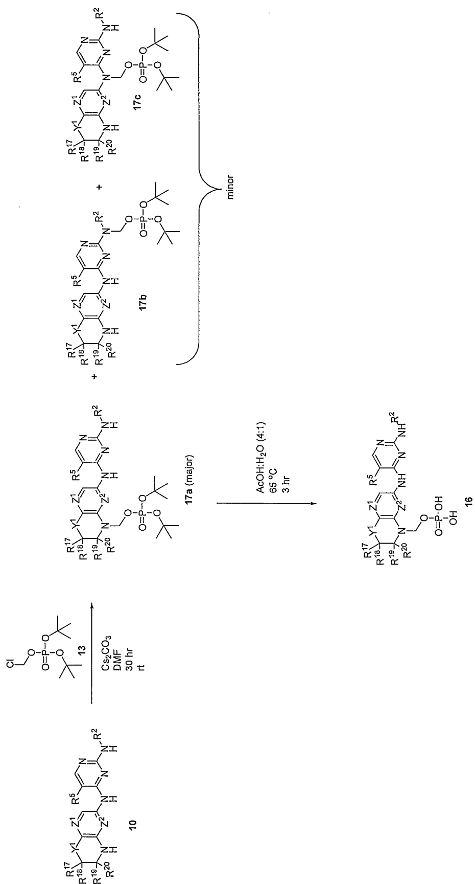
Scheme (V)
