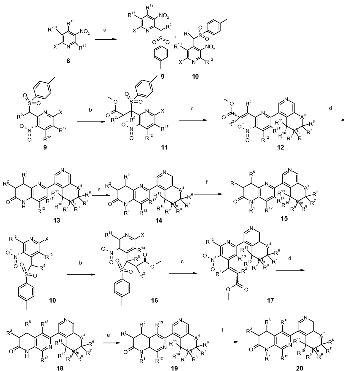
Scheme 1b
