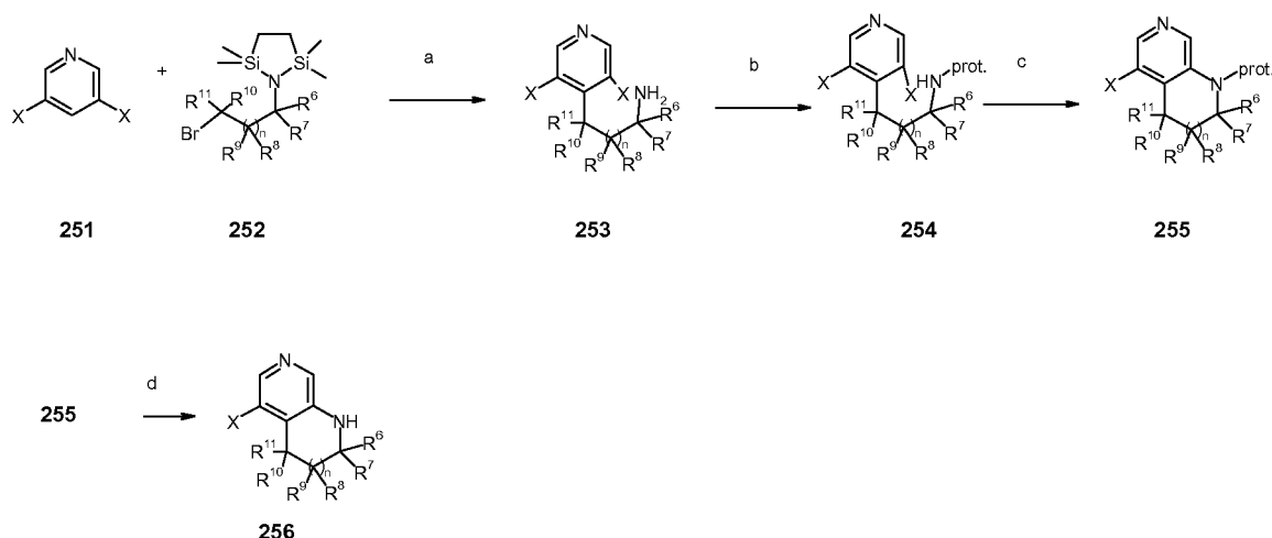
Scheme 3b
