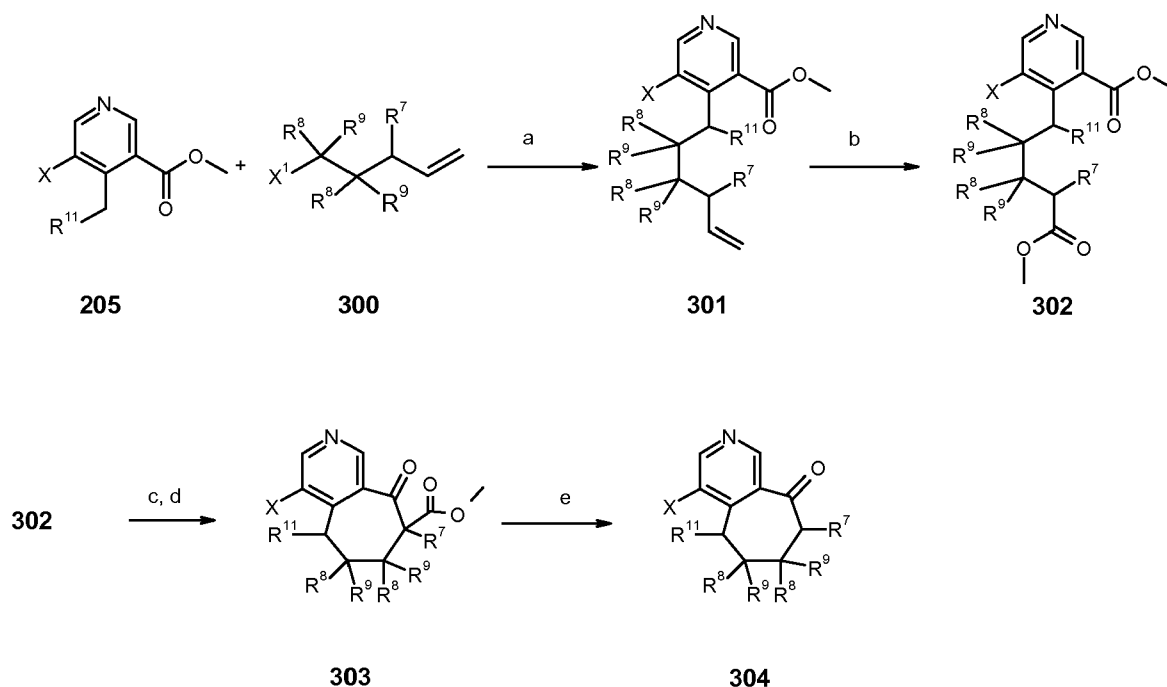
Scheme 3c
