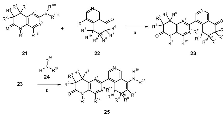
Scheme 1c
