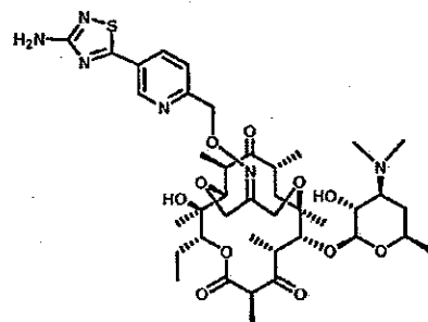
Compound 2
