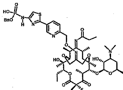
Compound 9
