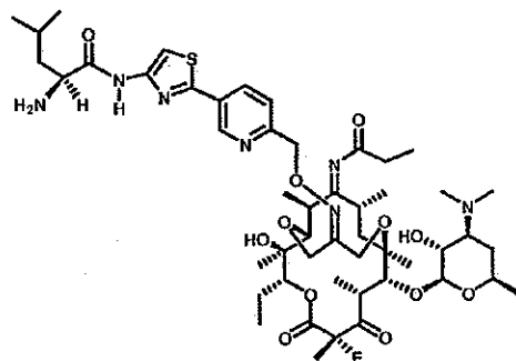
Compound 6
