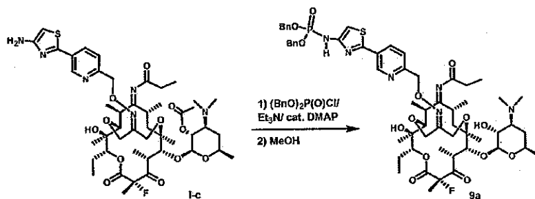
Compound 9
