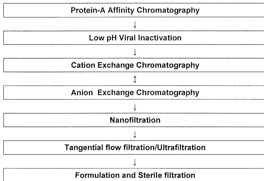
Figure 1 : Flow chart - Downstream processing for purification of monoclonal antibody
