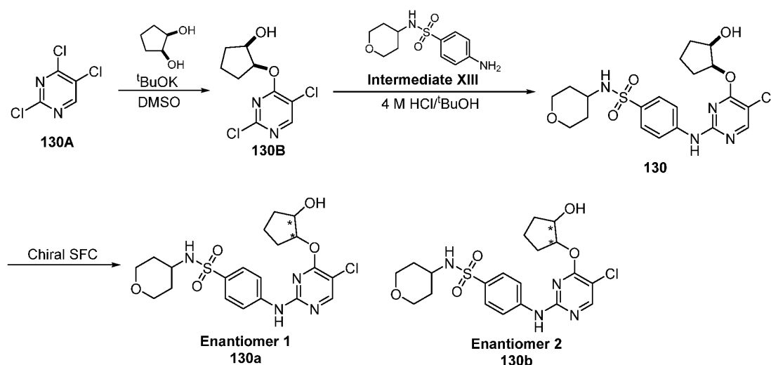
Illustration 18. Synthesis of 4-((5-chloro-4-((2-hydroxycyclopentyl)oxy)pyrimidin-2-yl)amino)-N-(tetrahydro-2H-pyran-4-yl)benzenesulfonamide ( 130 )
