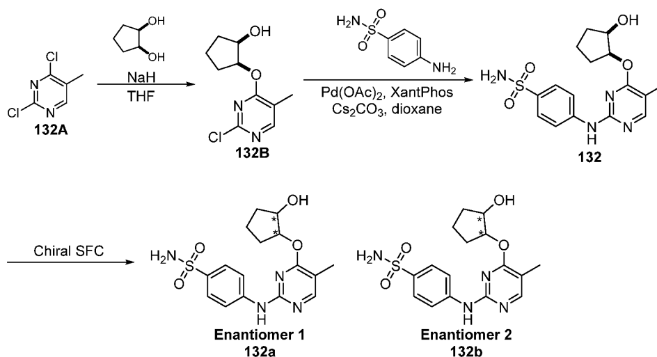
Illustration 20. Synthesis of cis -4-((4-((2-hydroxycyclopentyl)oxy)-5-methylpyrimidin-2-yl)amino)benzenesulfonamide ( 132 )
