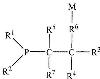
Formula IV
