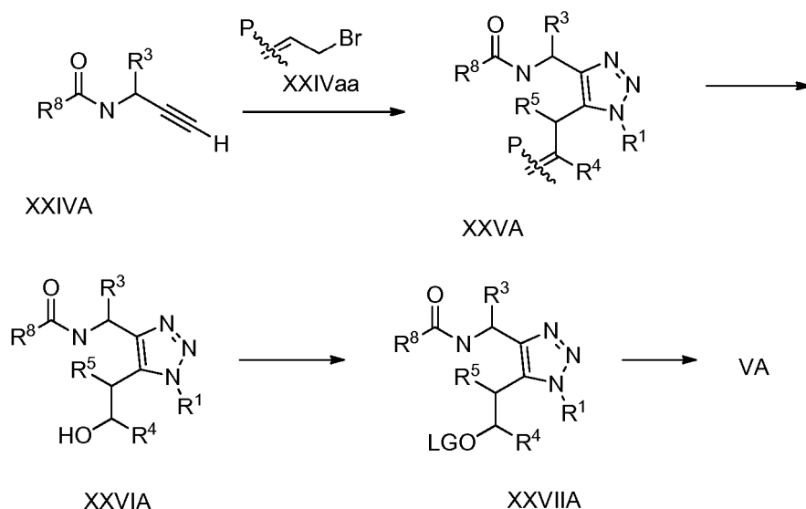
Scheme 8
