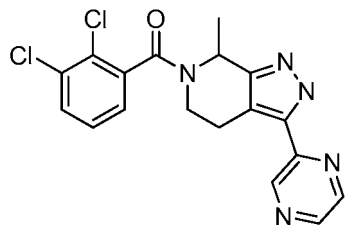
Example 433: (2,3-dichlorophenyl)(7-methyl-3-(pyrazin-2-yl)-4,5-dihydro-2H-pyrazolo[3,4-c]pyridin-6(7H)-yl)methanone.
