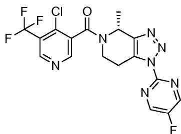
Example 340: (R*)-(3-chloro-2-(trifluoromethyl)pyridin-4-yl)(1-(5-fluoropyrimidin-2-yl)-4-methyl-6,7-dihydro-1H-[1,2,3]triazolo[4,5-c]pyridin-5(4H)-yl)methanone
