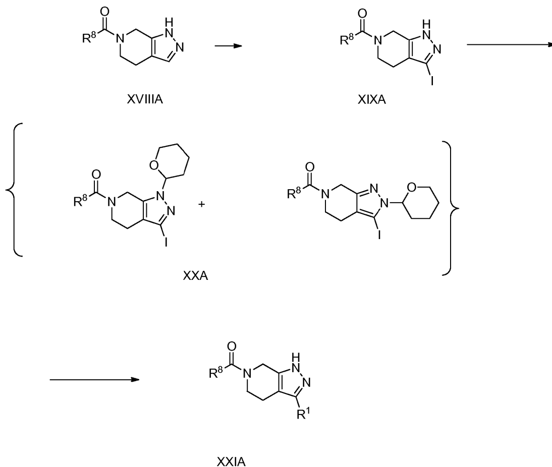
Scheme 6
