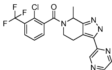
Example 439: (S*)-(2-chloro-3-(trifluoromethyl)phenyl)(4-methyl-1-(4-methylpyrimidin-2-yl)-6,7-dihydro-1H-[1,2,3]triazolo[4,5-c]pyridin-5(4H)-yl)methanone
