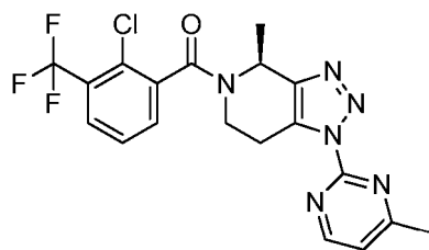
Example 439: (S*)-(2-chloro-3-(trifluoromethyl)phenyl)(4-methyl-1-(4-methylpyrimidin-2-yl)-6,7-dihydro-1H-[1,2,3]triazolo[4,5-c]pyridin-5(4H)-yl)methanone
