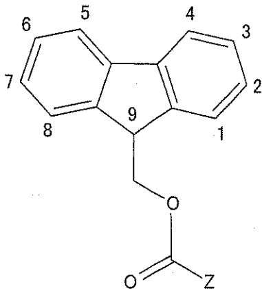
(formula 1)
