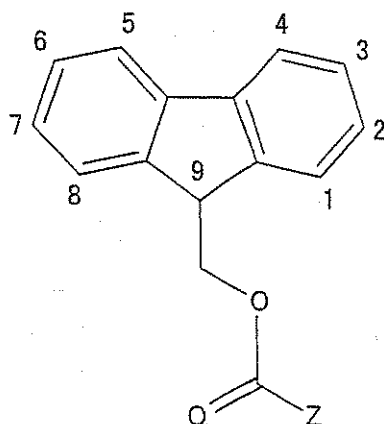
(formula 1)
