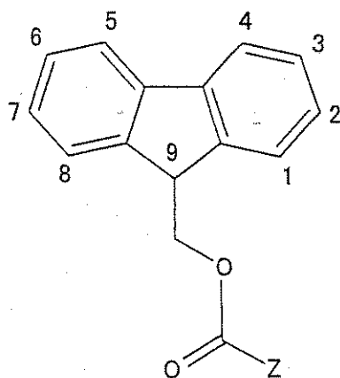
(formula 1)
