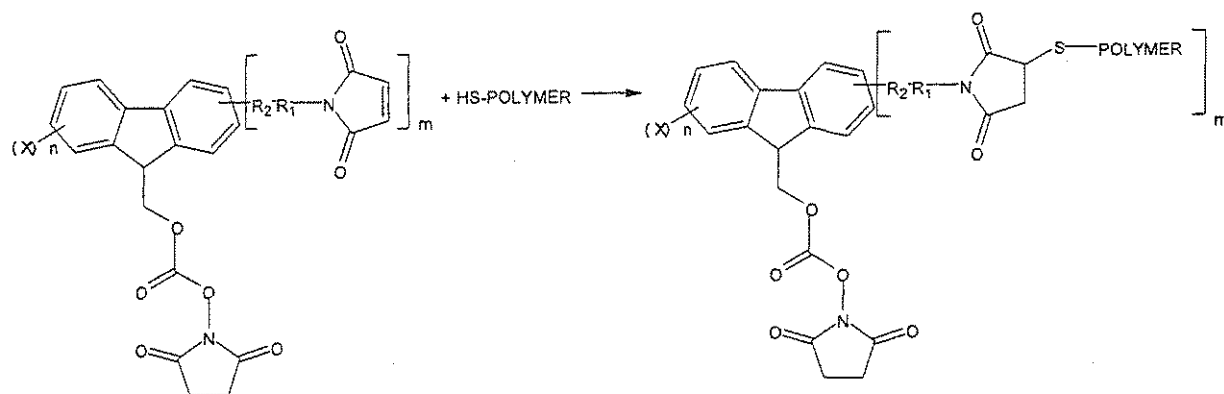
(formula 2)
