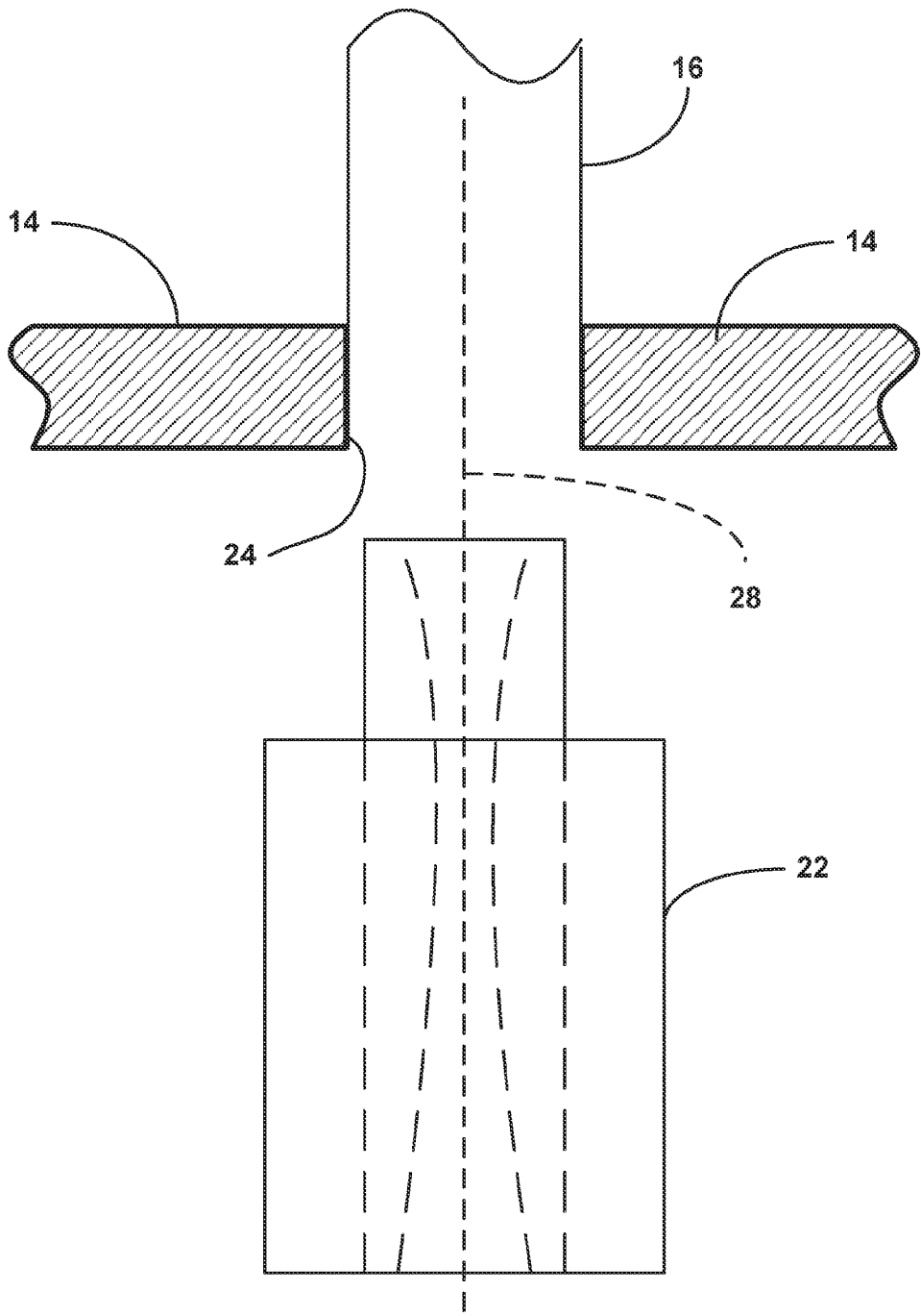
Fig 4 Prior Art
