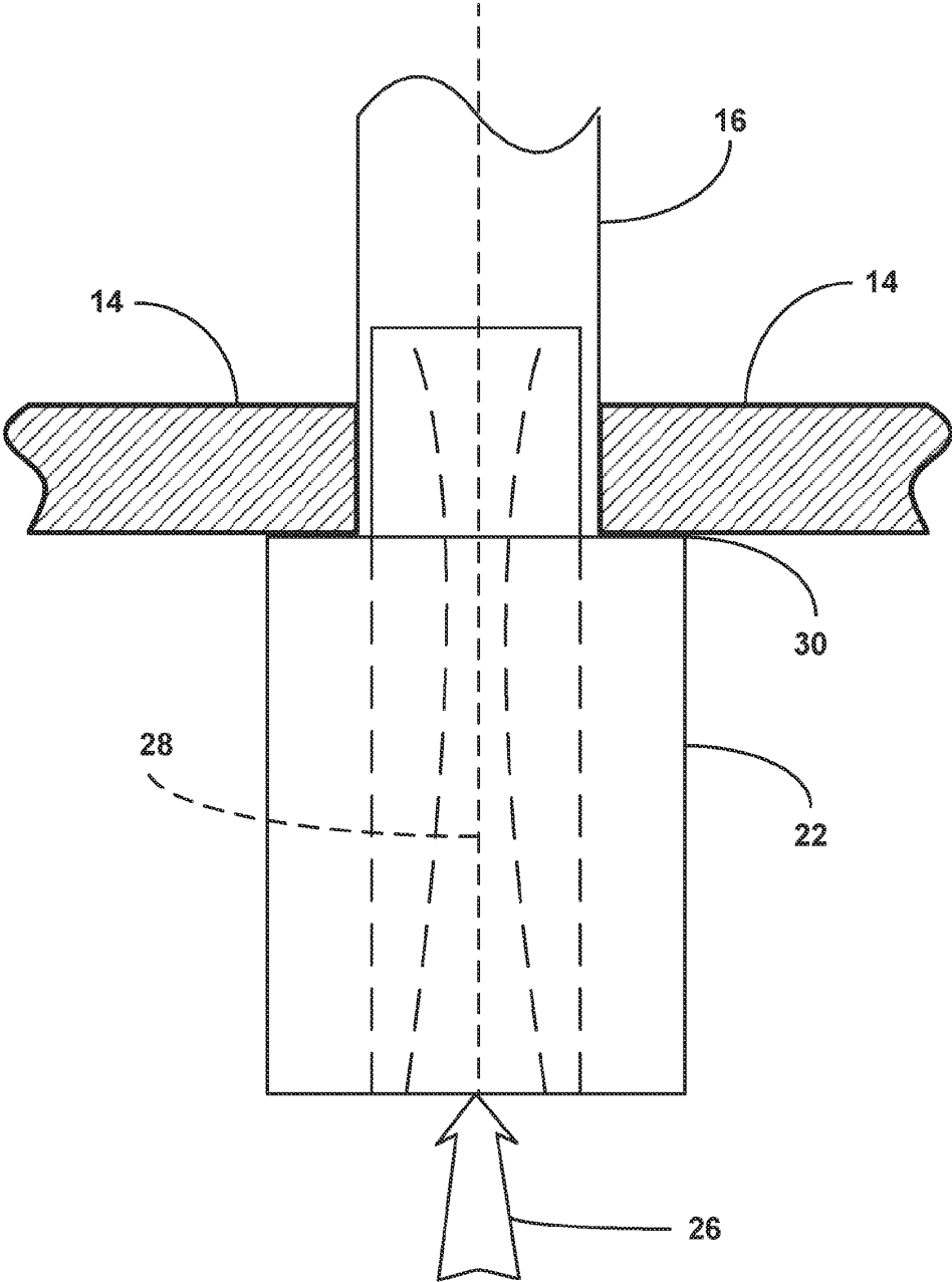
Fig 5 Prior Art
