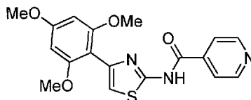
N -(4-(2,4,6-Trimethoxyphenyl)thiazol-2-yl)isonicotinamide compound II-11
