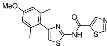
N -(4-(4-Methoxy-2,6-dimethylphenyl)thiazol-2-yl)thiazole-5-carboxamide compound II-75
