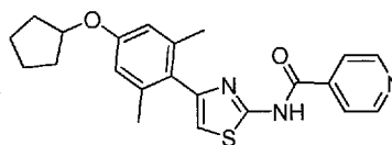
N -(4-(4-(Cyclopentyloxy)-2,6-dimethylphenyl)thiazol-2-yl)isonicotinamide compound II-85
