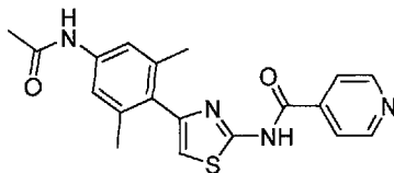
N -(4-(4-Acetamido-2,6-dimethylphenyl)thiazol-2-yl)isonicotinamide compound II-74
