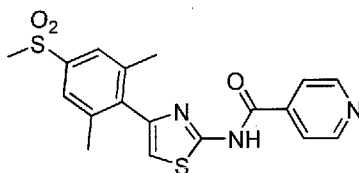
N -(4-(2,6-Dimethyl-4-(methylsulfonyl)phenyl)thiazol-2-yl)isonicotinamide compound II-127
