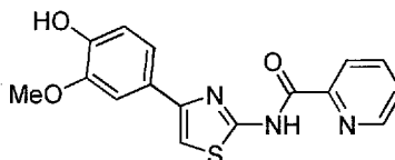
N -(4-(4-Hydroxy-3-methoxyphenyl)thiazol-2-yl)picolinamide compound II-36
