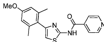
N -(4-(4-Methoxy-2,6-dimethylphenyl)thiazol-2-yl)isonicotinamide compound II-42
