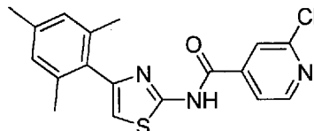
2-Chloro-N-(4-mesitylthiazol-2-yl)isonicotinamide compound II-64
