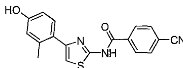
4-Cyano- N -(4-(4-hydroxy-2-methylphenyl)thiazol-2-yl)benzamide compound II-61
