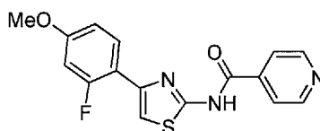
N -(4-(2-Fluoro-4-methoxyphenyl)thiazol-2-yl)isonicotinamide compound II-26
