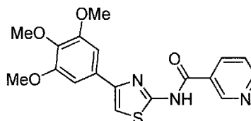
N -(4-(3,4,5-Trimethoxyphenyl)thiazol-2-yl)nicotinamide compound II-20
