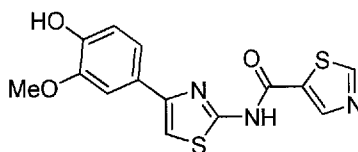
N -(4-(4-Hydroxy-3-methoxyphenyl)thiazol-2-yl)thiazole-5-carboxamide compound II-50
