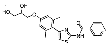
N -(4-(4-(2,3-Dihydroxypropoxy)-2,6-dimethylphenyl)thiazol-2-yl)isonicotinamide compound II-97
