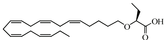
(S)-2-((5Z,8Z,11Z,14Z,17Z)-icosa-5,8,11,14,17-pentaenyloxy)butanoic acid;
