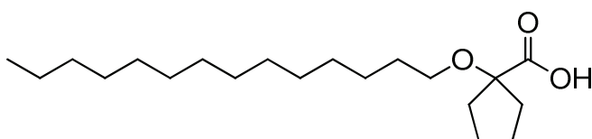
2-ethyl-2-(tetradecyloxy)butanoic acid (2)
