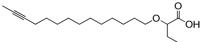
2-(tetradec-12-ynyloxy)butanoic acid ( 52 )
