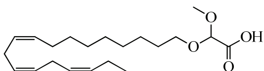
2-methoxy-2-((9Z,12Z,15Z)-octadeca-9,12,15-trien-1-yloxy)acetic acid ( 29 )
