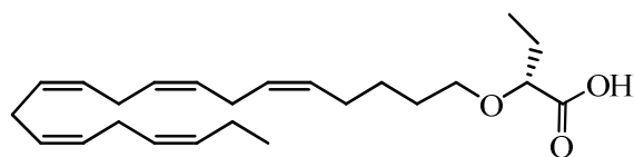
(R)-2-((5Z,8Z,11Z,14Z,17Z)-icosa-5,8,11,14,17-pentaenyloxy)butanoic acid;
