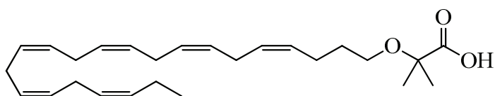
2-((4Z,7Z,10Z,13Z,16Z,19Z)-docosa-4,7,10,13,16,19-hexaen-1-yloxy)-2-methylpropanoic acid ( 22 )
