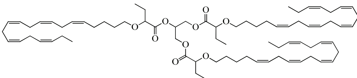
propane-1,2,3-triyl tris(2-((5Z,8Z,11Z,14Z,17Z)-icosa-5,8,11,14,17-pentaen-1-yloxy)butanoate) ( 43 )
