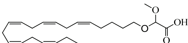
2-((5Z,8Z,11Z,14Z,17Z)-icosa-5,8,11,14,17-pentaen-1-yloxy)-2-methoxyacetic acid (17)
