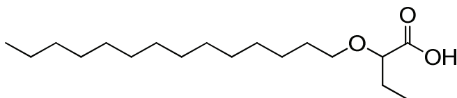
2-(Tetradecyloxy)butanoic acid (1)
