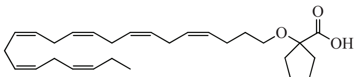
2-((4Z,7Z,10Z,13Z,16Z,19Z)-docosa-4,7,10,13,16,19-hexaen-1-yloxy)-2-ethylbutanoic acid ( 20 )
