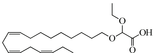
2-ethoxy-2-((9Z,12Z,15Z)-octadeca-9,12,15-trien-1-yloxy)acetic acid ( 30 )
