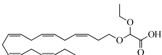
2-ethoxy-2-((3Z,6Z,9Z,12Z,15Z)-octadeca-3,6,9,12,15-pentaen-1-yloxy)acetic acid ( 42 )
