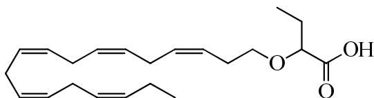
2-((3Z,6Z,9Z,12Z,15Z)-octadeca-3,6,9,12,15-pentaen-1-yloxy)butanoic acid (37)
