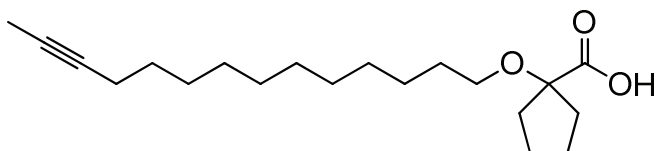
2-ethyl-2-(tetradec-12-yn-1-yloxy)butanoic acid ( 53 )
