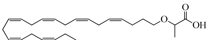
2-((4Z,7Z,10Z,13Z,16Z,19Z)-docosa-4,7,10,13,16,19-hexaen-1-yloxy)propanoic acid ( 21 )
