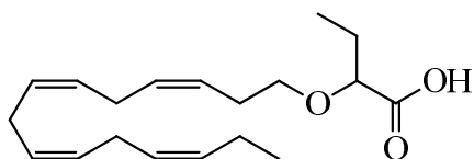
2-((3Z,6Z,9Z,12Z)-pentadeca-3,6,9,12-tetraen-1-yloxy)butanoic acid ( 31 )
