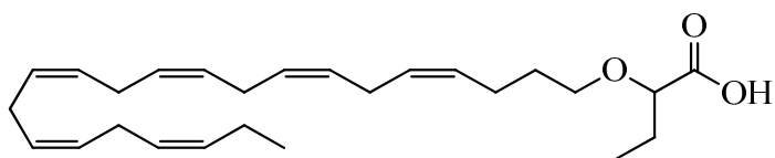
2-((4Z,7Z,10Z,13Z,16Z,19Z)-docosa-4,7,10,13,16,19-hexaen-1-yloxy)butanoic acid ( 19 )
