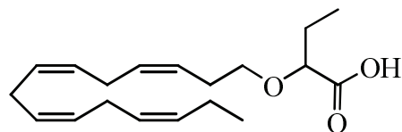
2-((3Z,6Z,9Z,12Z)-pentadeca-3,6,9,12-tetraenyloxy)butanoic acid;
