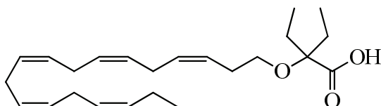
2-ethyl-2-((3Z,6Z,9Z,12Z,15Z)-octadeca-3,6,9,12,15-pentaen-1-yloxy)butanoic acid (38)
