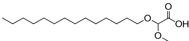
2-methoxy-2-(tetradecyloxy)acetic acid (5)
