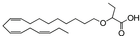
2-((9Z,12Z,15Z)-octadeca-9,12,15-trienyloxy)butanoic acid;
