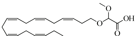
2-methoxy-2-((3Z,6Z,9Z,12Z,15Z)-octadeca-3,6,9,12,15-pentaen-1-yloxy)acetic acid ( 41 )
