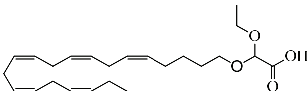
2-ethoxy-2-((5Z,8Z,11Z,14Z,17Z)-icosa-5,8,11,14,17-pentaen-1-yloxy)acetic acid (18)
