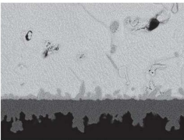
Ref.4: Sn-17In-2.5Ag-1.5Bi
