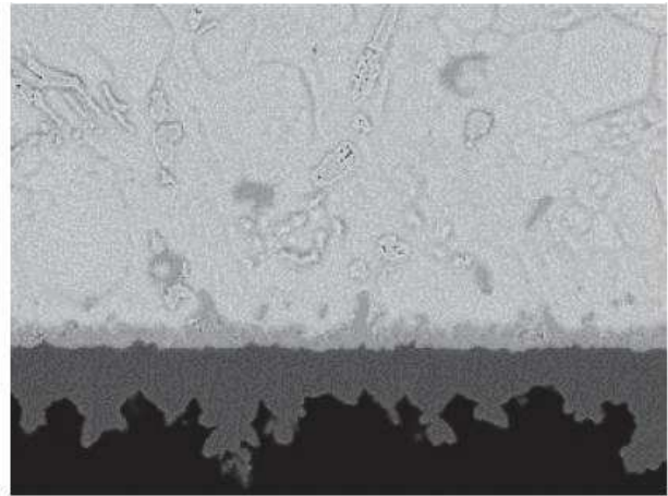
Ex.2: Sn-15.0In-2.5Ag-2.0Bi-0.02Ni
