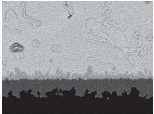
Ex.3: Sn-17In-2.5Ag-1.5Bi-0.02Ni
