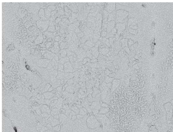
Ex.3: Sn-17In-2.5Ag-1.5Bi-0.02Ni
