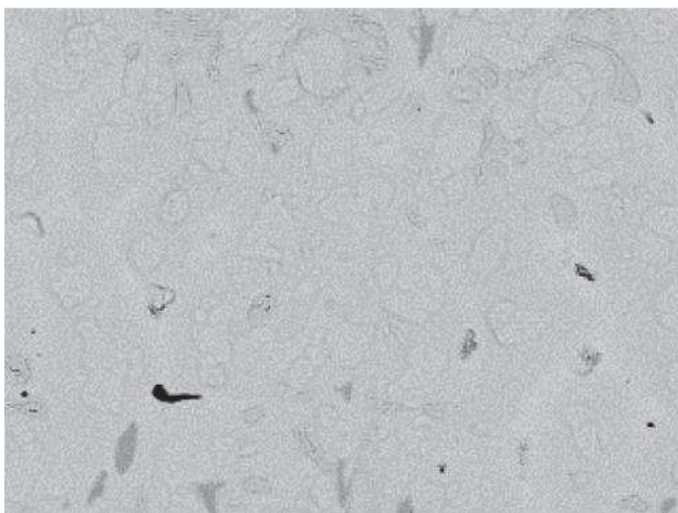
Ref.2: Sn-15.0In-2.5Ag-2.0Bi
