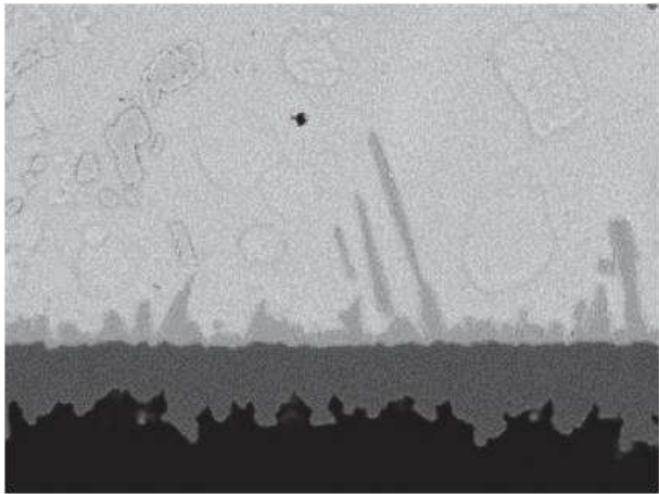
Ref.2: Sn-15.0In-2.5Ag-2.0Bi
