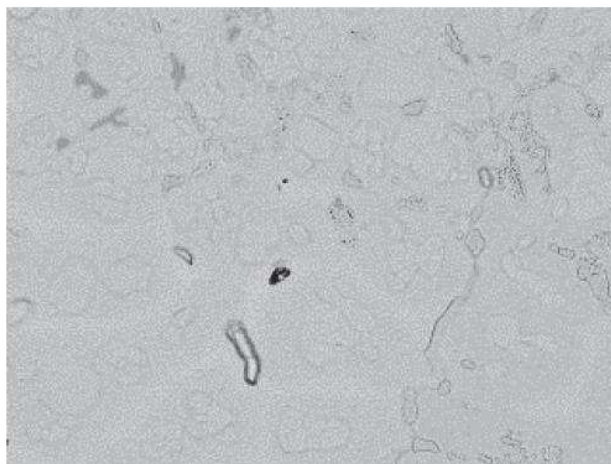
Ex.2: Sn-15.0In-2.5Ag-2.0Bi-0.02Ni
