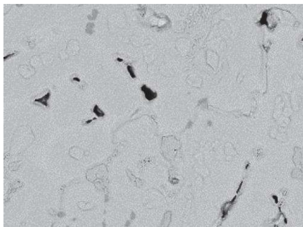
Ref.4: Sn-17In-2.5Ag-1.5Bi
