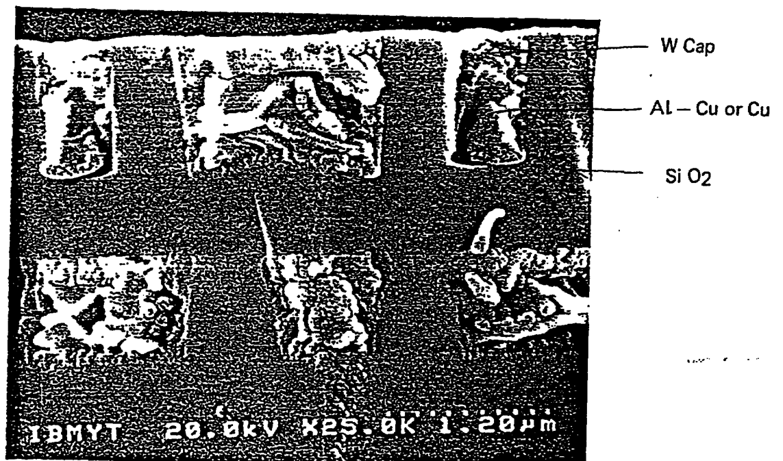
AFTER POLISHING CVD W AND THE LOW RESISTIVITY METAL.
