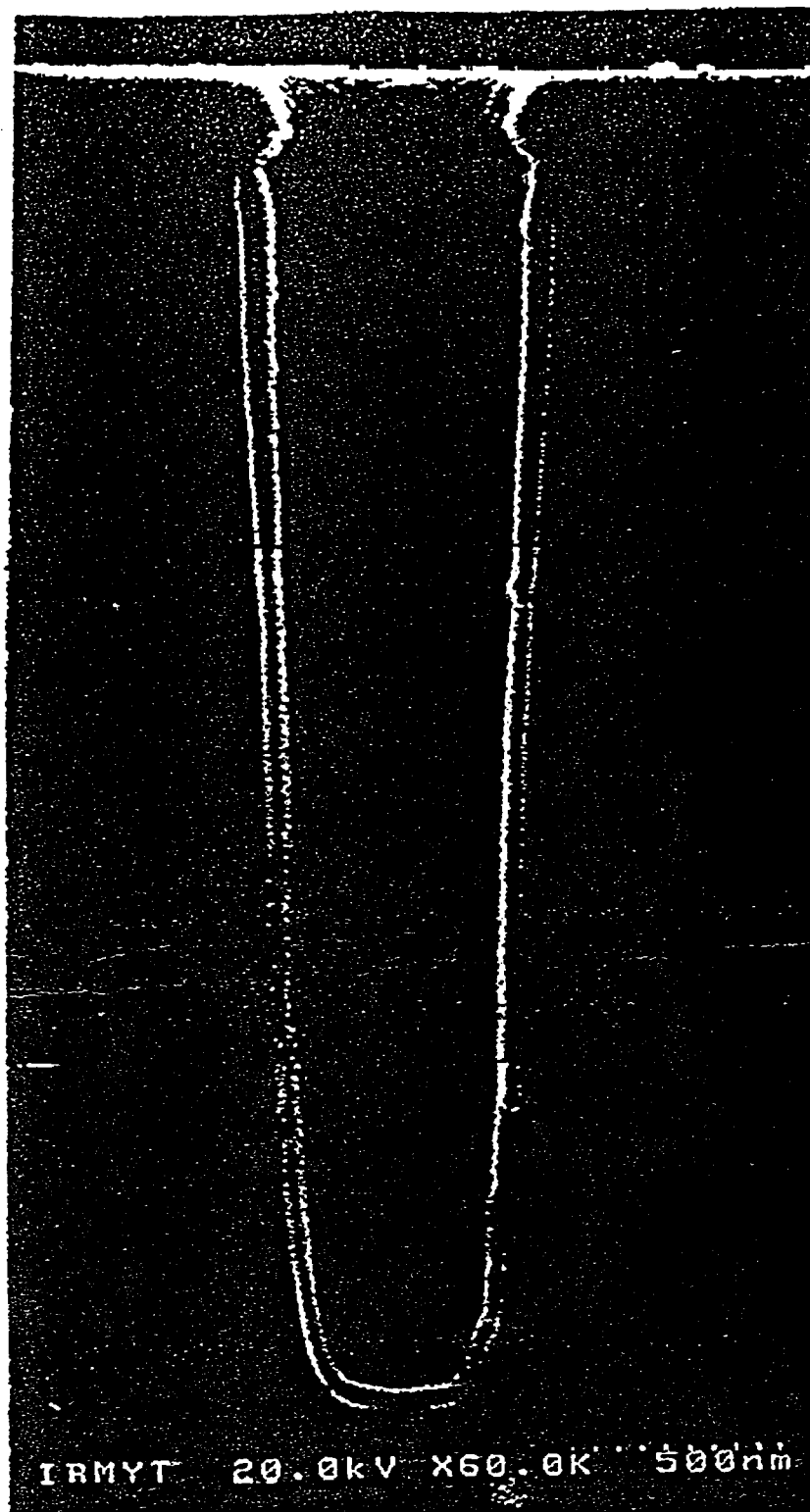
SEM of liner applied by collimated sputtering prior to CVD of Tungsten
