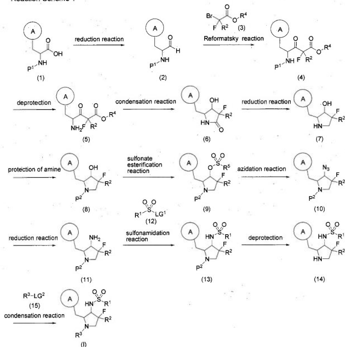
Reaction Scheme 1
