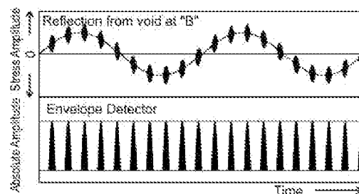
Figure 3c, Detection of Linear Scatterer with Envelope Detector
