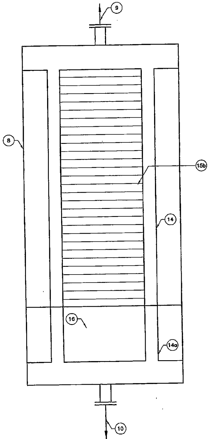
FIGURE 2c. THREE PHASE SEPARATOR (TOP VIEW)
