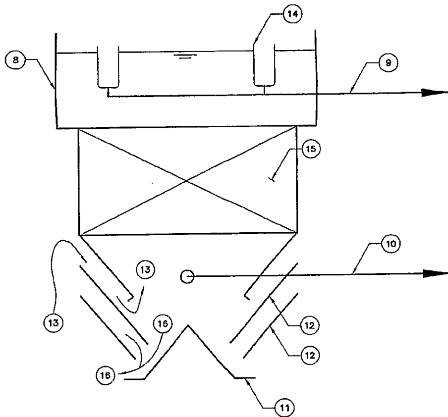
FIGURE 2a. THREE PHASE SEPARATOR
