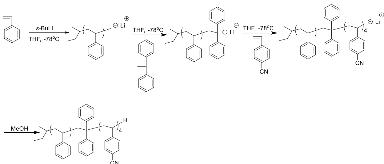
Scheme 4
