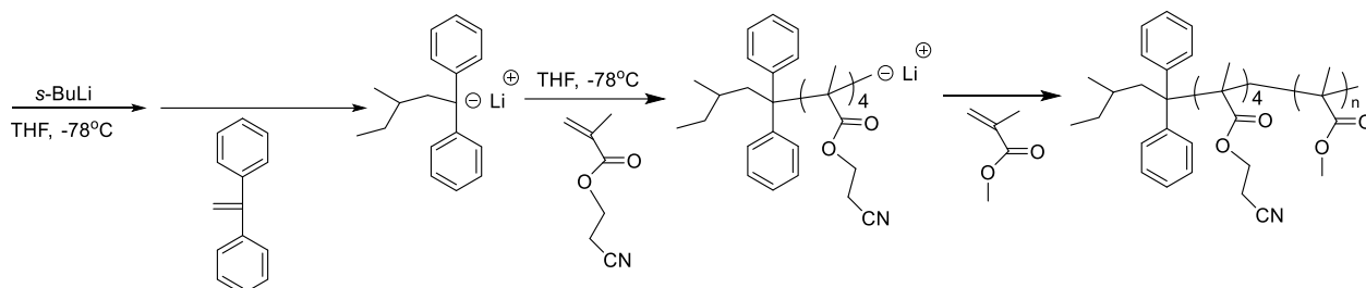
Scheme 6
