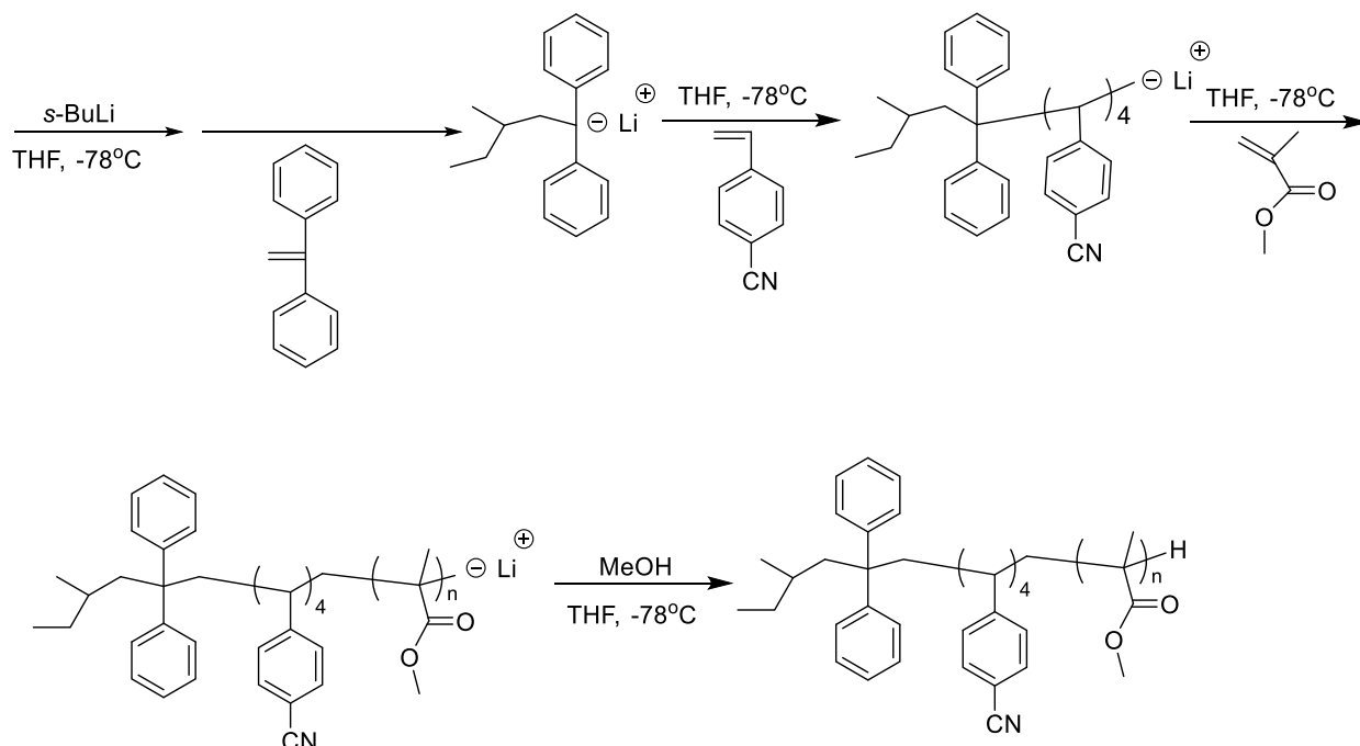
Scheme 5
