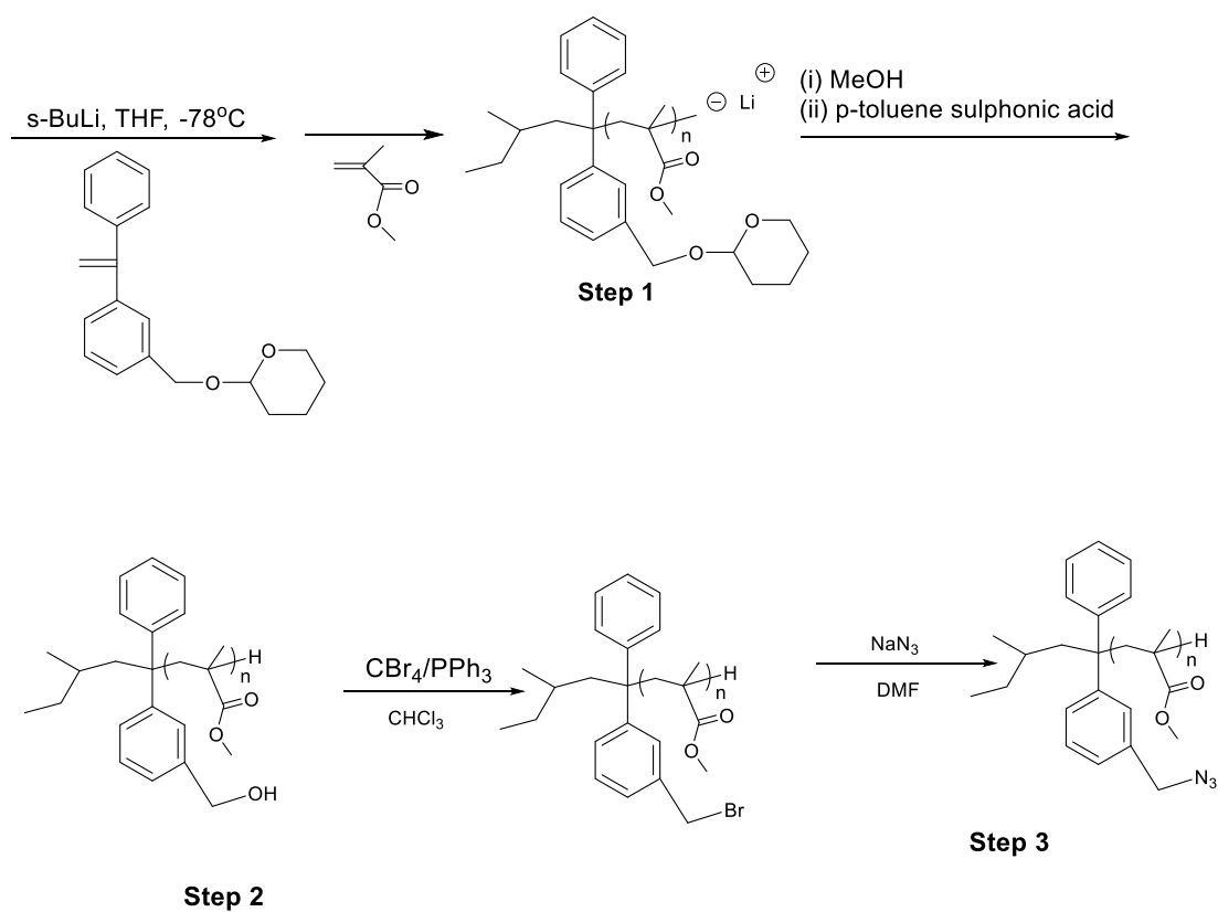
Scheme 2
