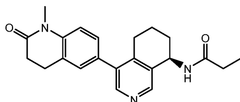
(R)-Compound 1
