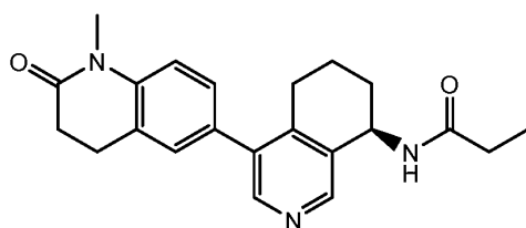
(R)-Compound 1.
