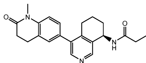
(R)-Compound 1.
