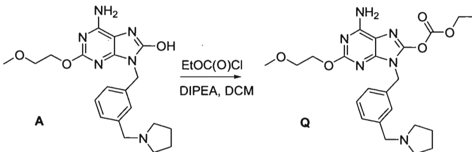
Scheme 4
