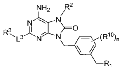
IIa
