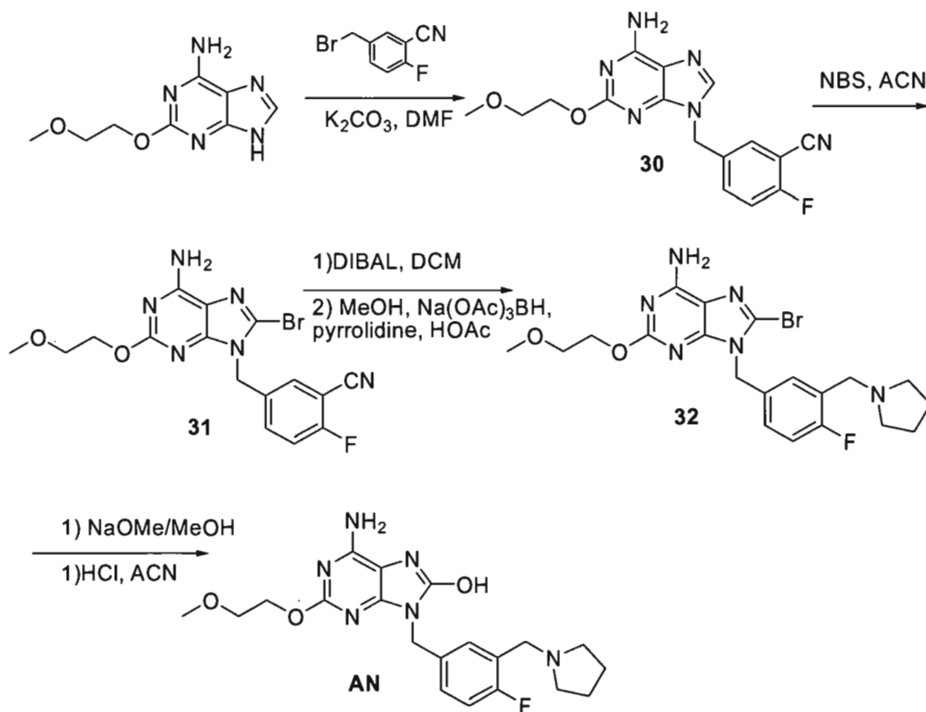
Scheme 16
