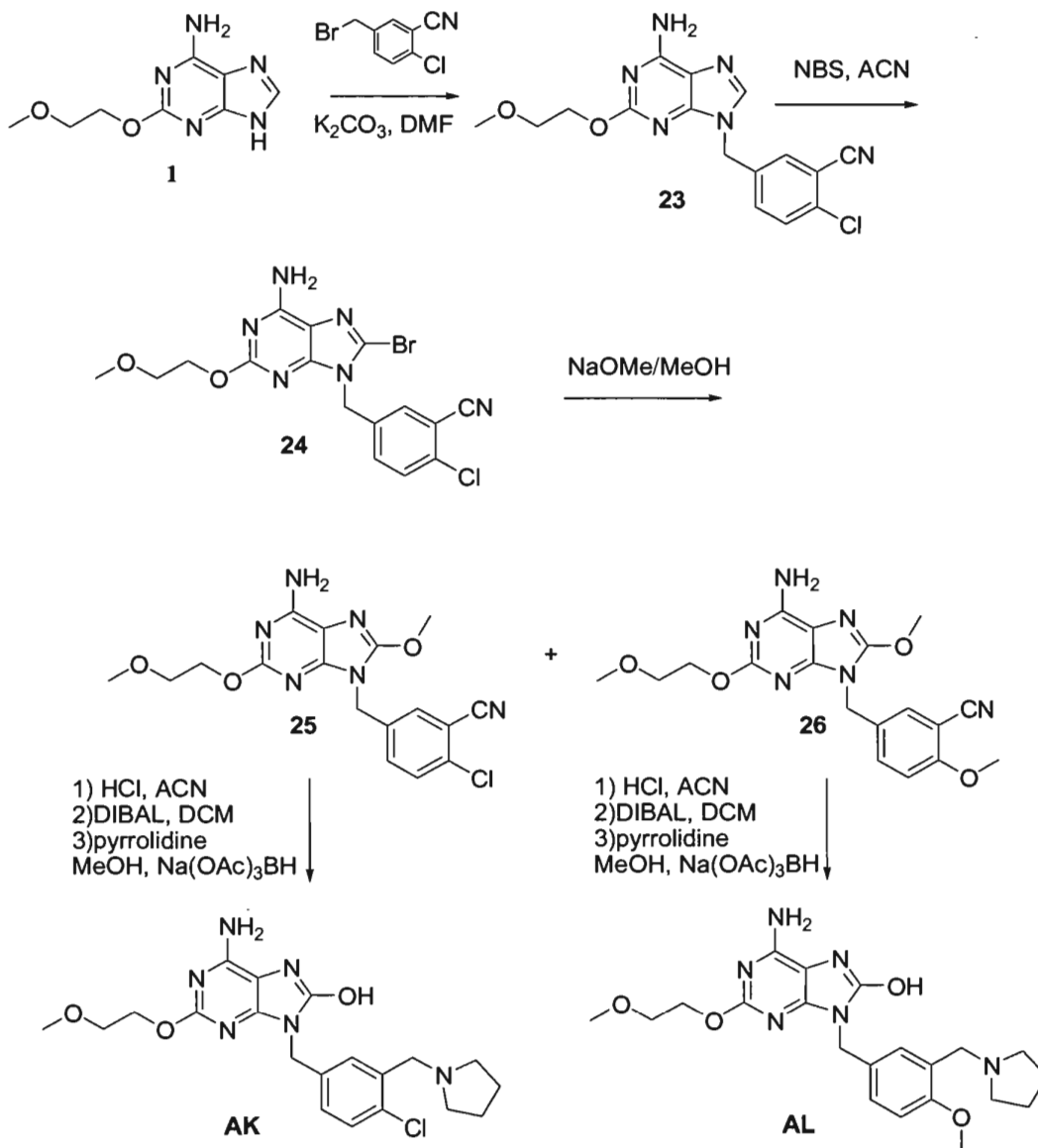
Scheme 14
