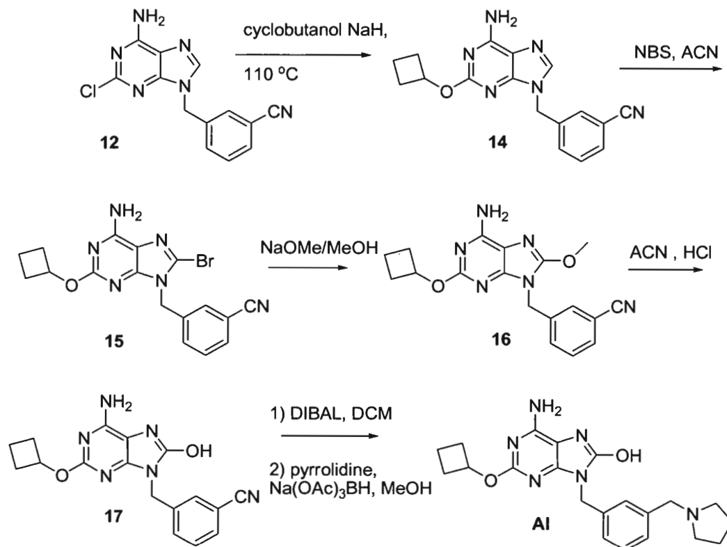
Scheme 12
