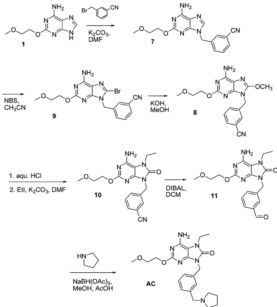
Scheme 10
