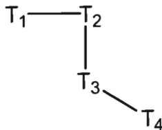
Formula III.
