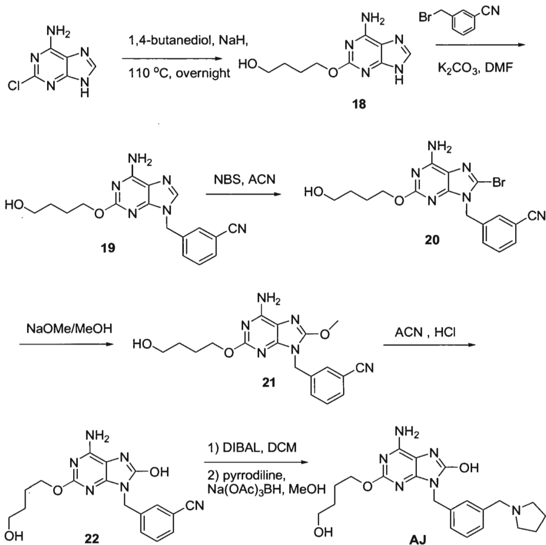
Scheme 13
