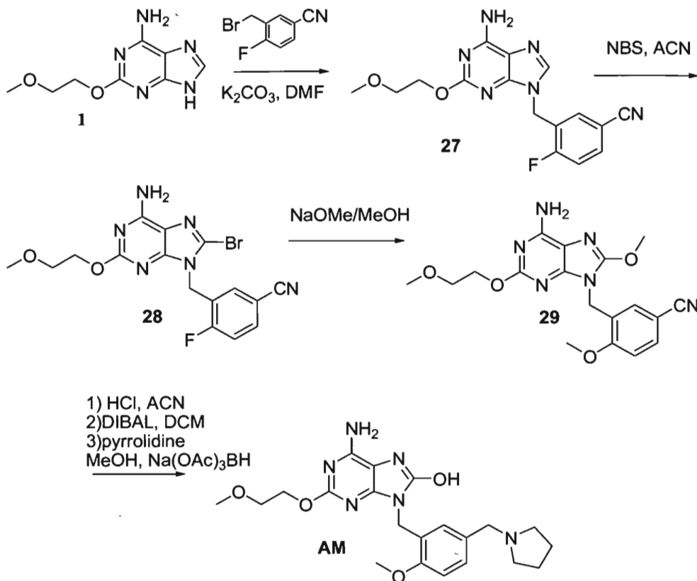
Scheme 15
