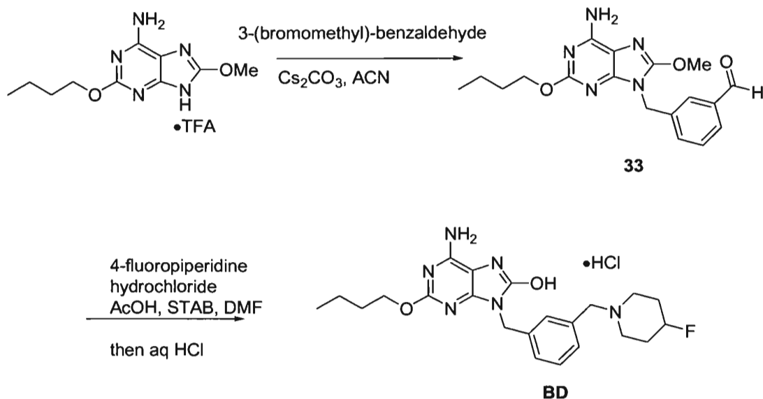
Scheme 17
