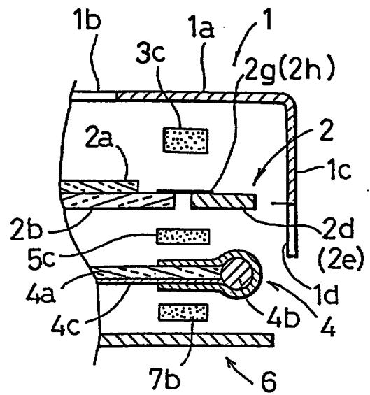
Fig.13 (Prior Art)
