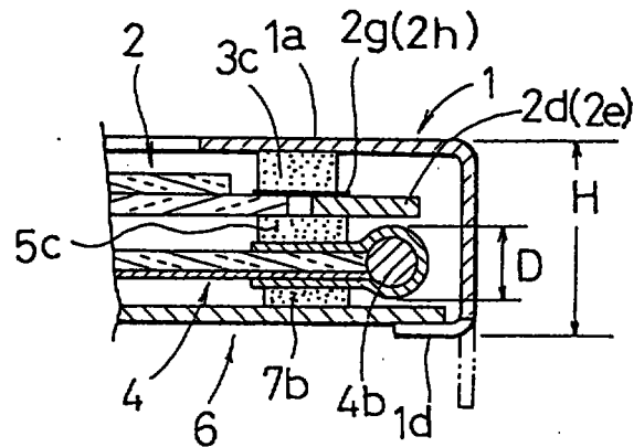
Fig.15 (Prior Art)
