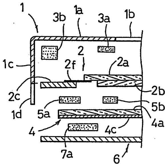
Fig.12 (Prior Art)
