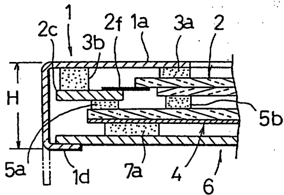
Fig.14 (Prior Art)
