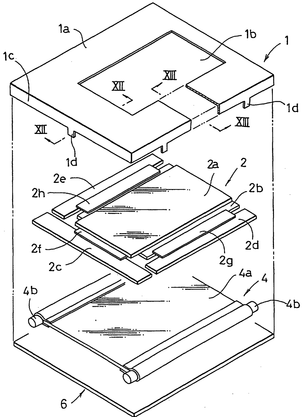
Fig.11 (Prior Art)
