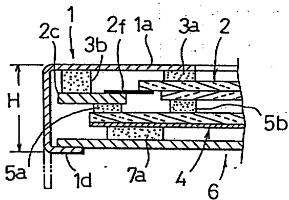
Fig.14 (Prior Art)
