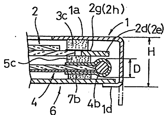
Fig.15 (Prior Art)
