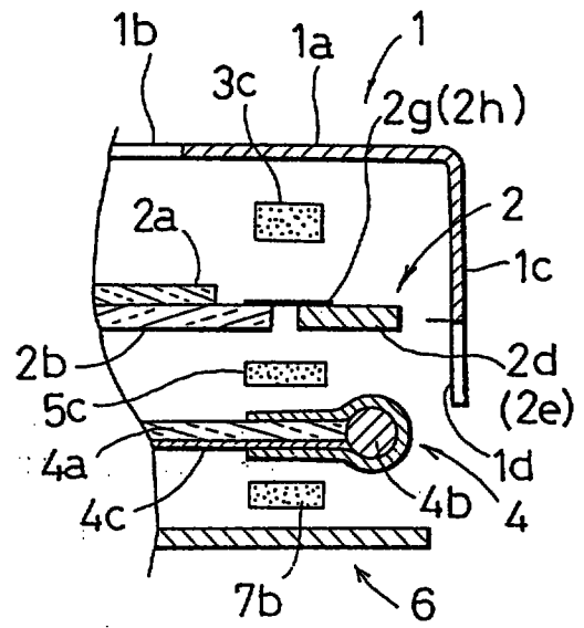
Fig.13 (Prior Art)
