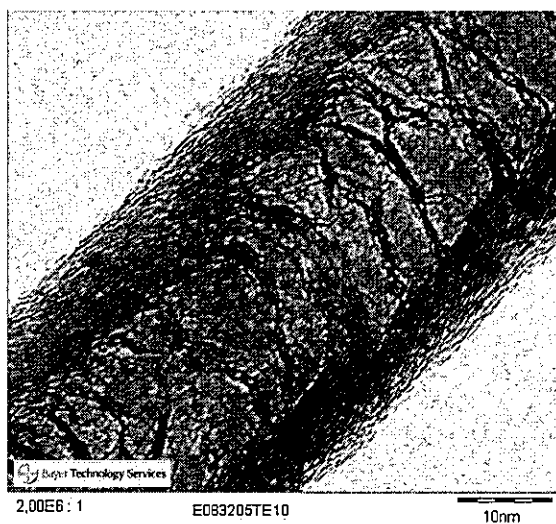
5 Fig. 2: Transmission electron micrograph of nitrogen-doped carbon nanotubes from Example 6
