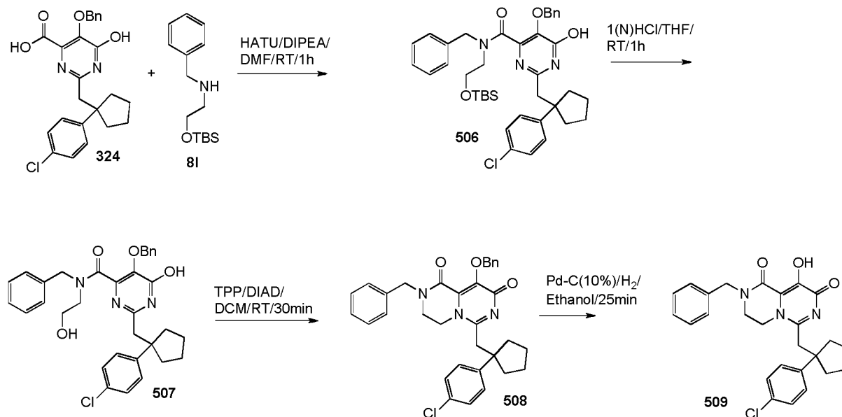
Scheme 52
