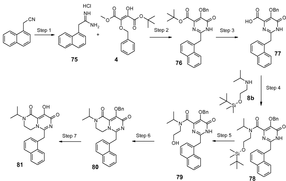
Scheme 13
