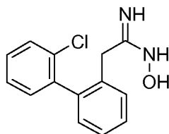
2-(2'-Chloro-biphenyl-2-yl)-N-hydroxy-acetamidine
