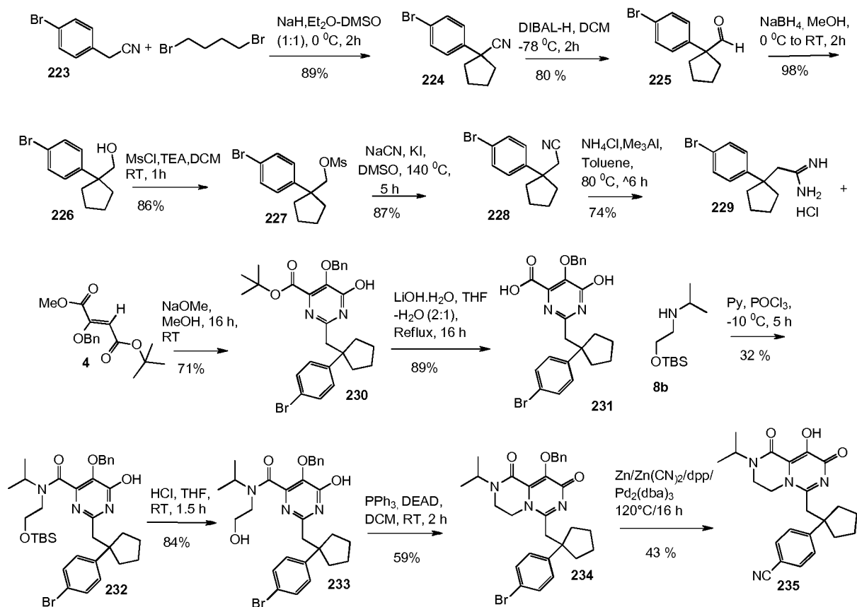
Scheme 39
