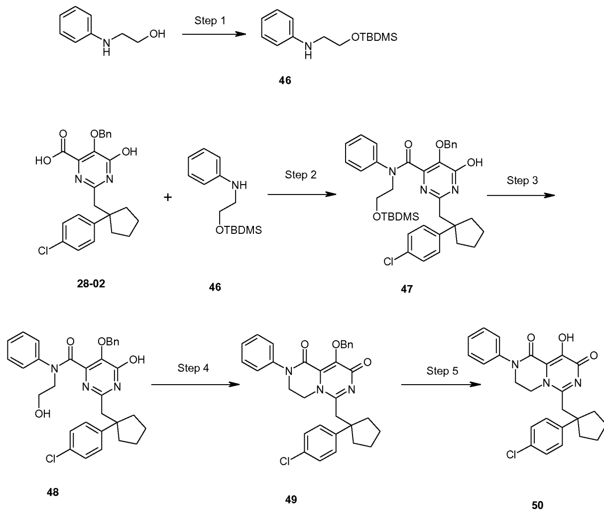
Scheme 9
