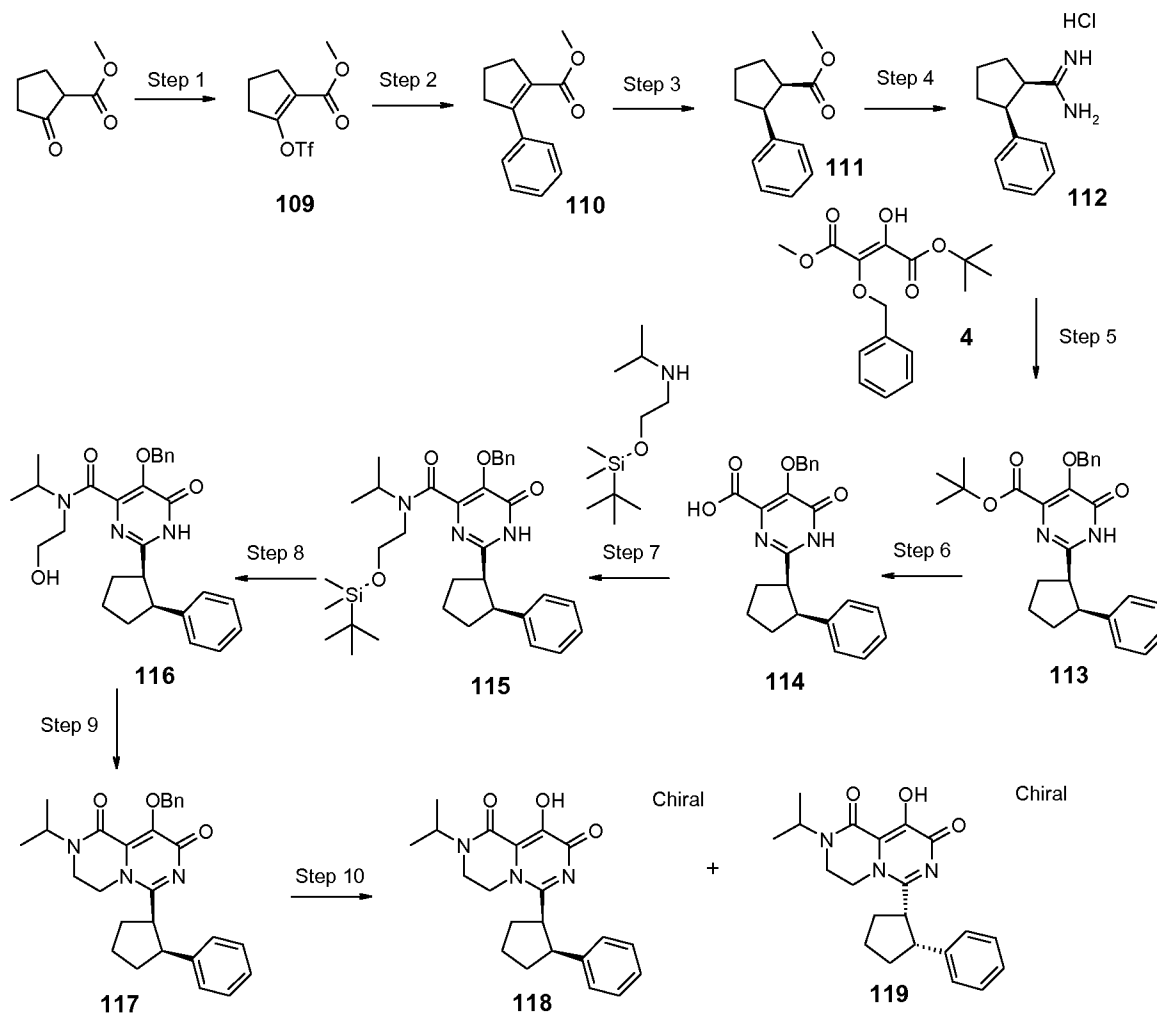
Scheme 17
