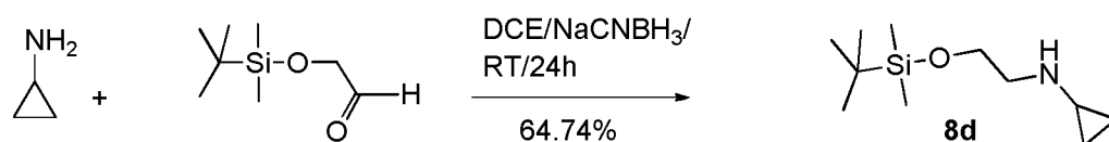
Scheme 45
