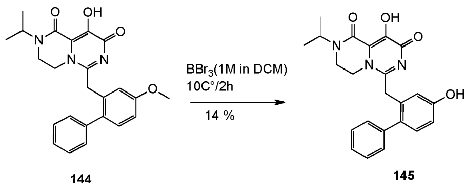
Scheme 20
