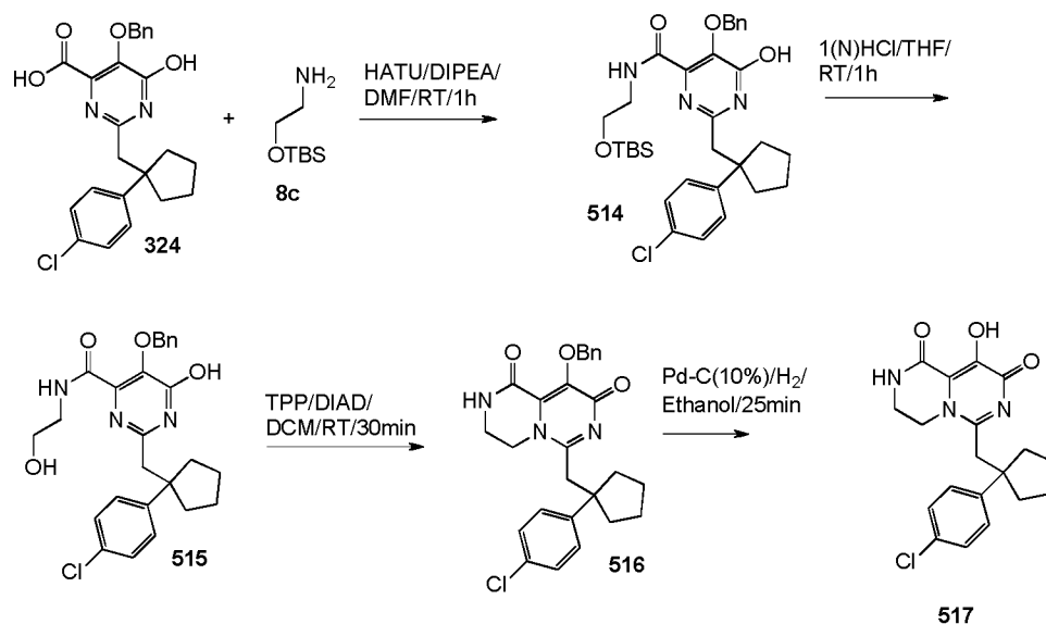
Scheme 53
