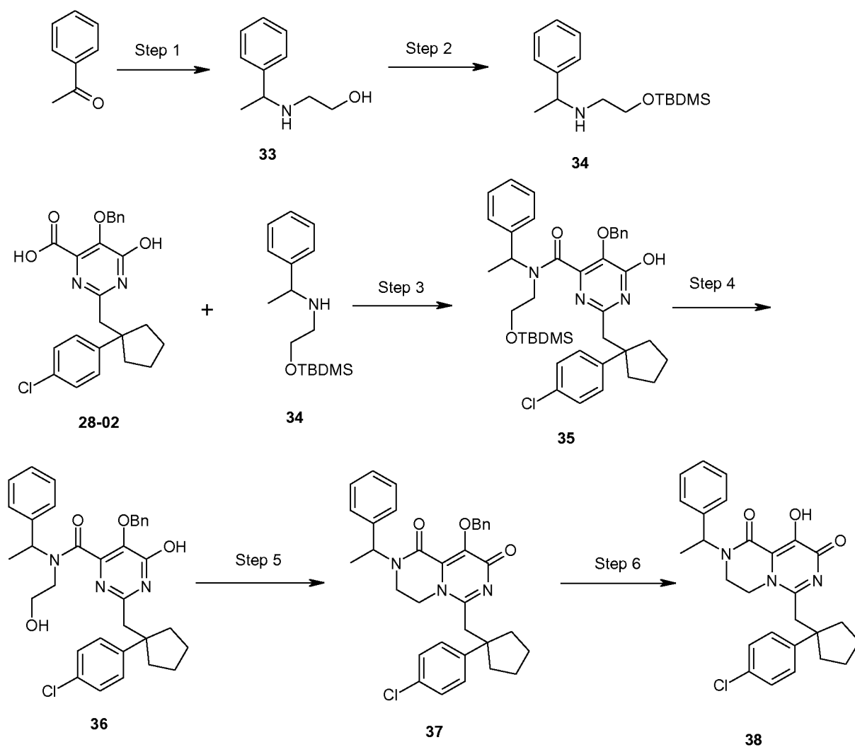
Scheme 7
