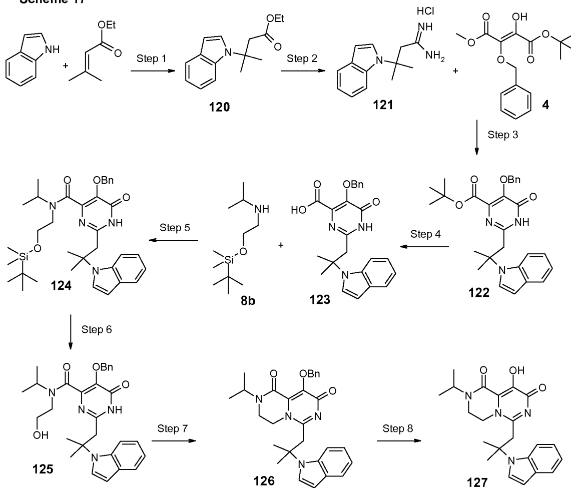
Scheme 17
