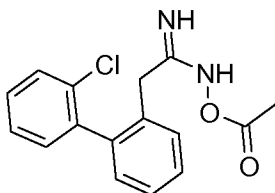
2-(2'-Chloro-biphenyl-2-yl)-N-acetyl-acetamidine
