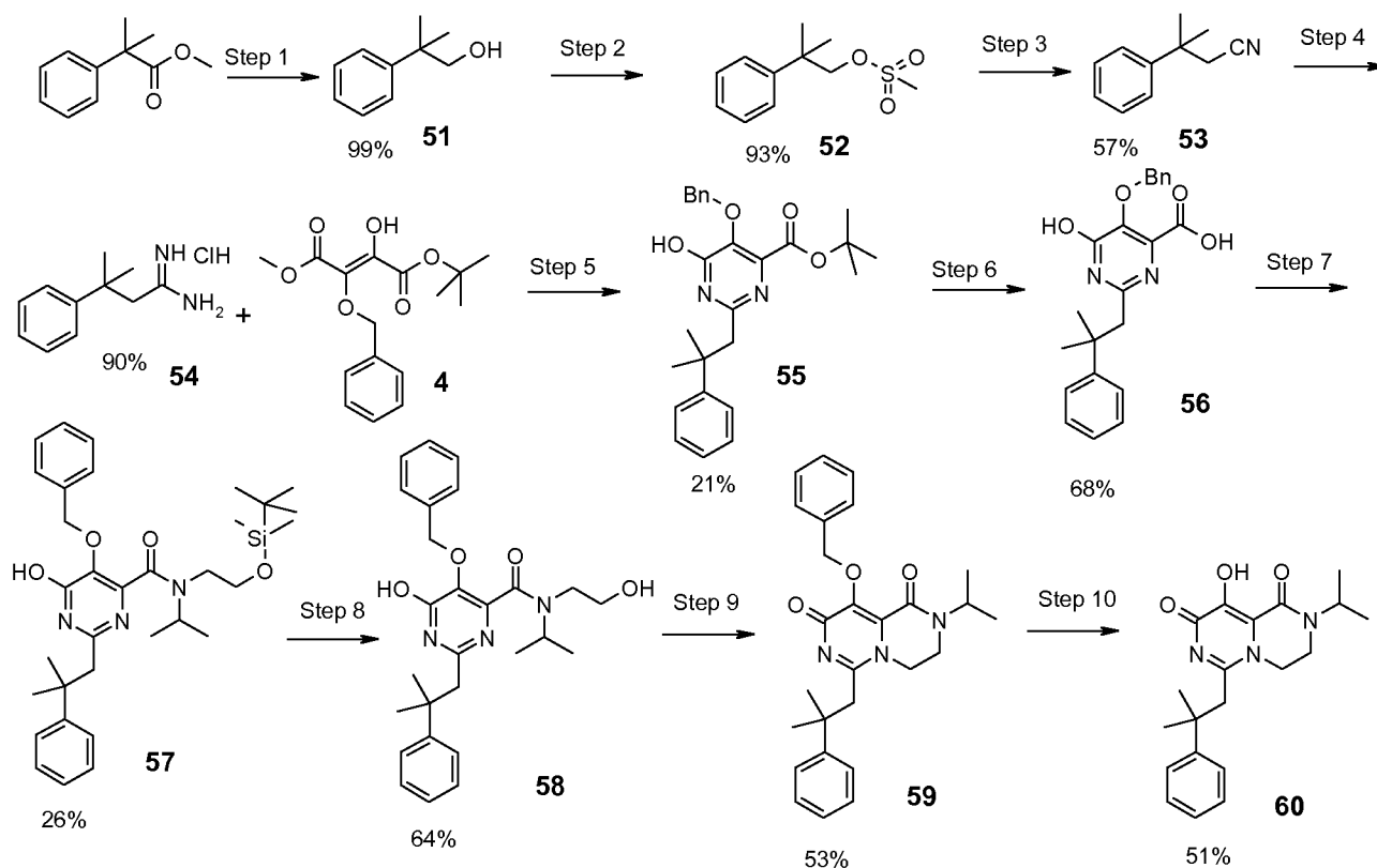
Scheme 10
