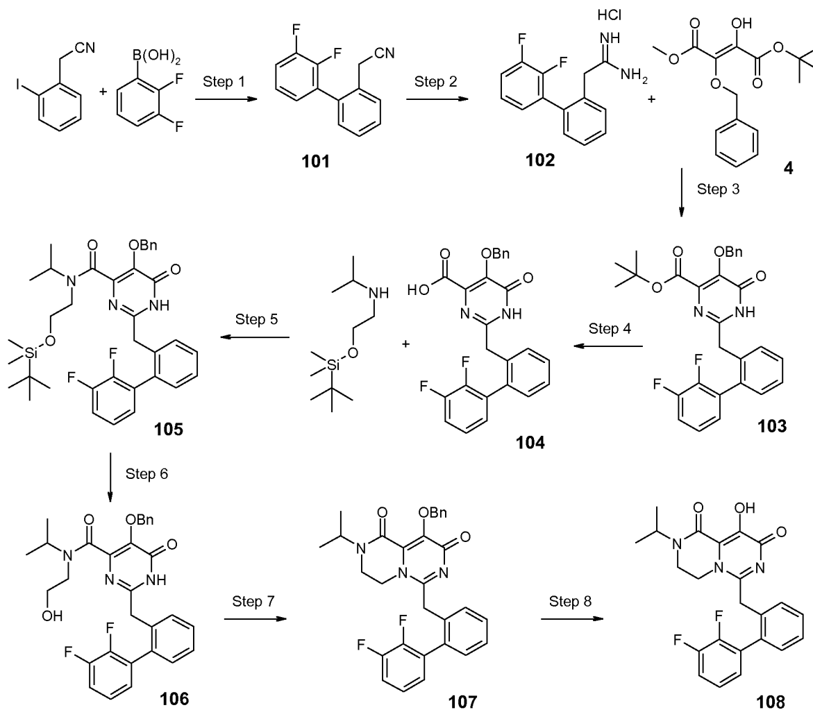
Scheme 16
