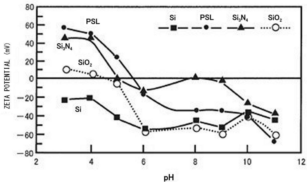
FIG. 1 PH VALUE DEPENDENCE OF ZETA POTENTIAL OF PSL PARTICULATE SURFACE, \text{SiO}_2 SURFACE, \text{Si}_3\text{N}_4 SURFACE, AND BARE Si SURFACE
