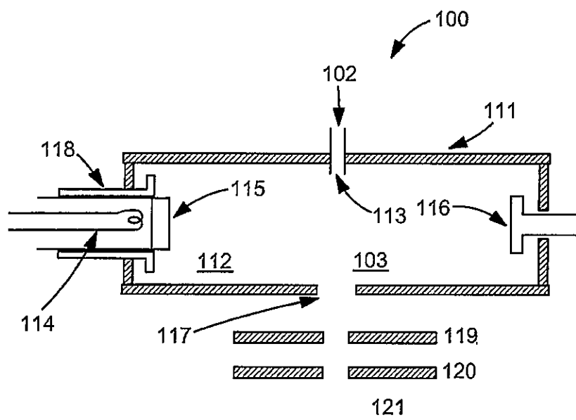
Schematic of an ion source apparatus
