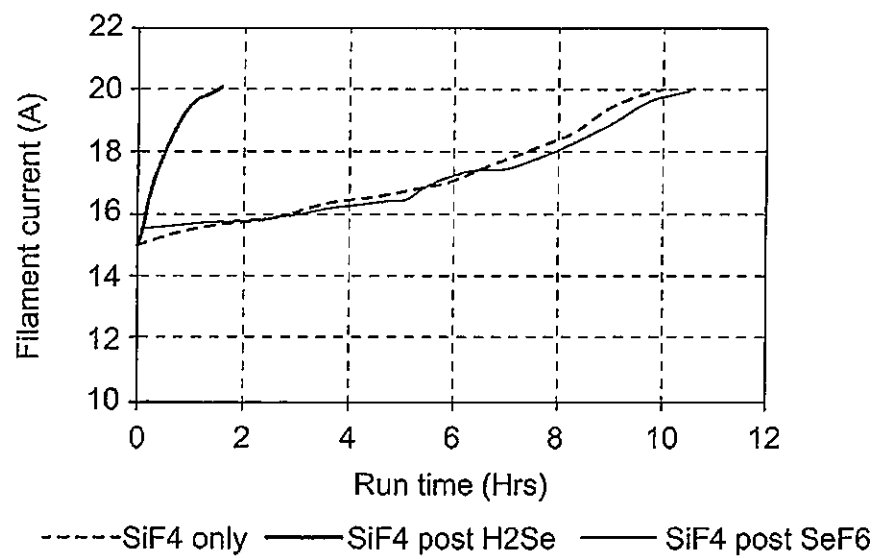
Filament current trend during SiF4 implant
