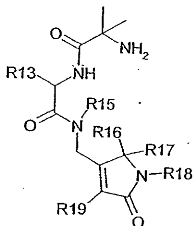
Formula V
