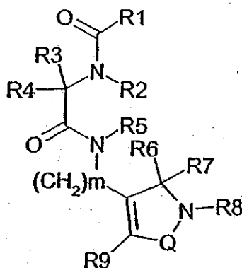
Formula II
