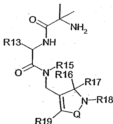
Formula III
