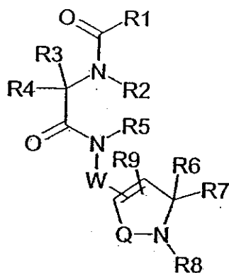
Formula I
