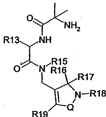
Formula III
