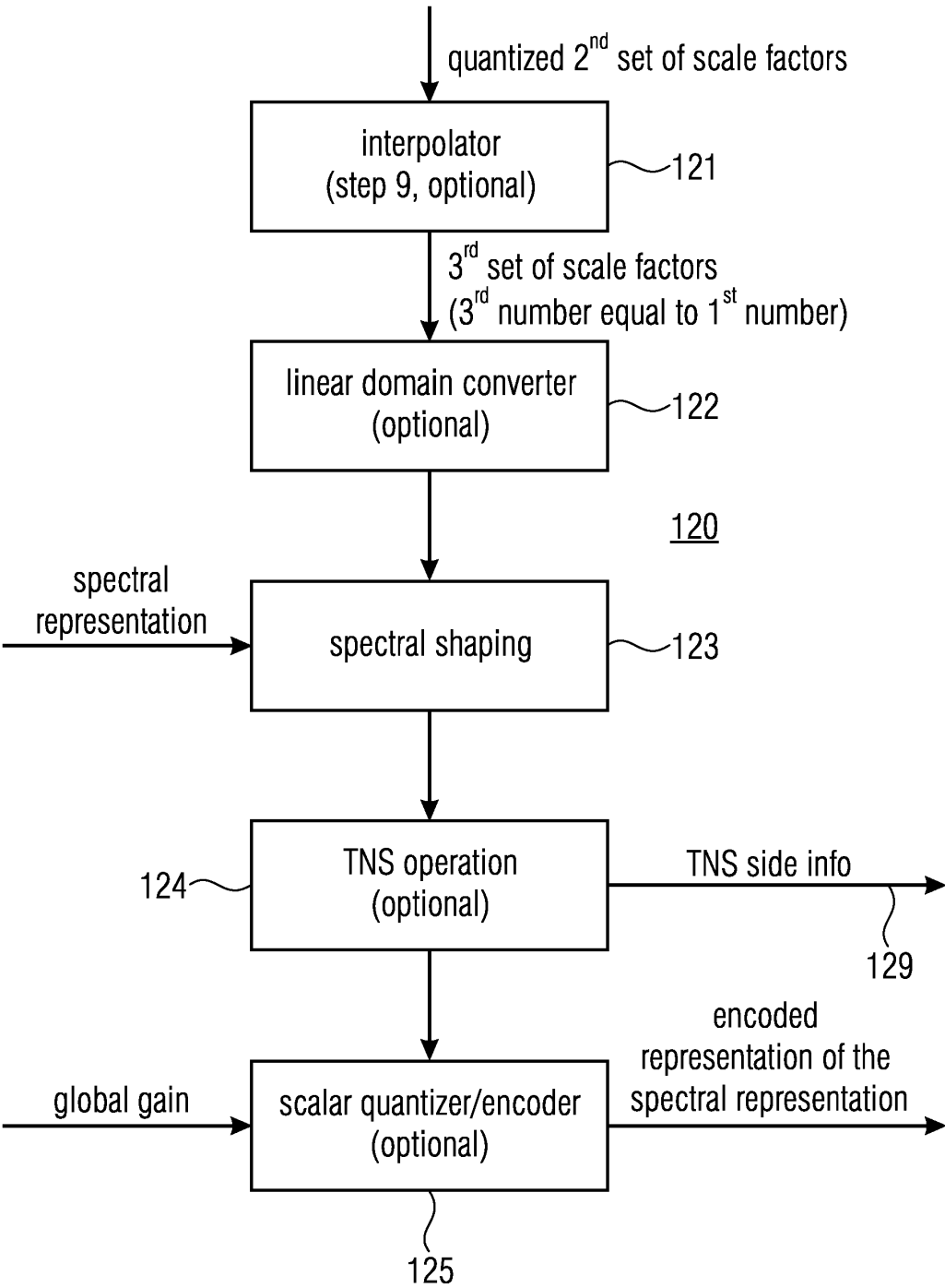
Fig. 5 (SPECTRAL PROCESSOR)
