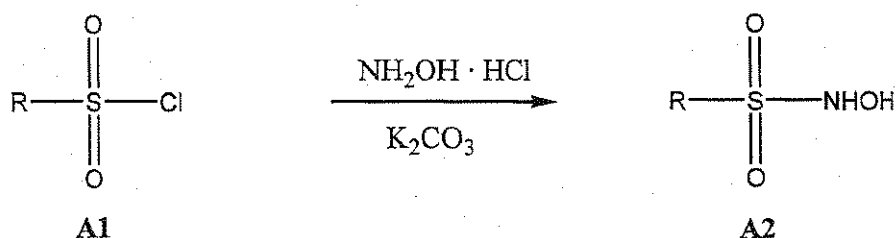
Scheme A. General Synthesis of N -Hydroxysulfonamides (Method 1).
